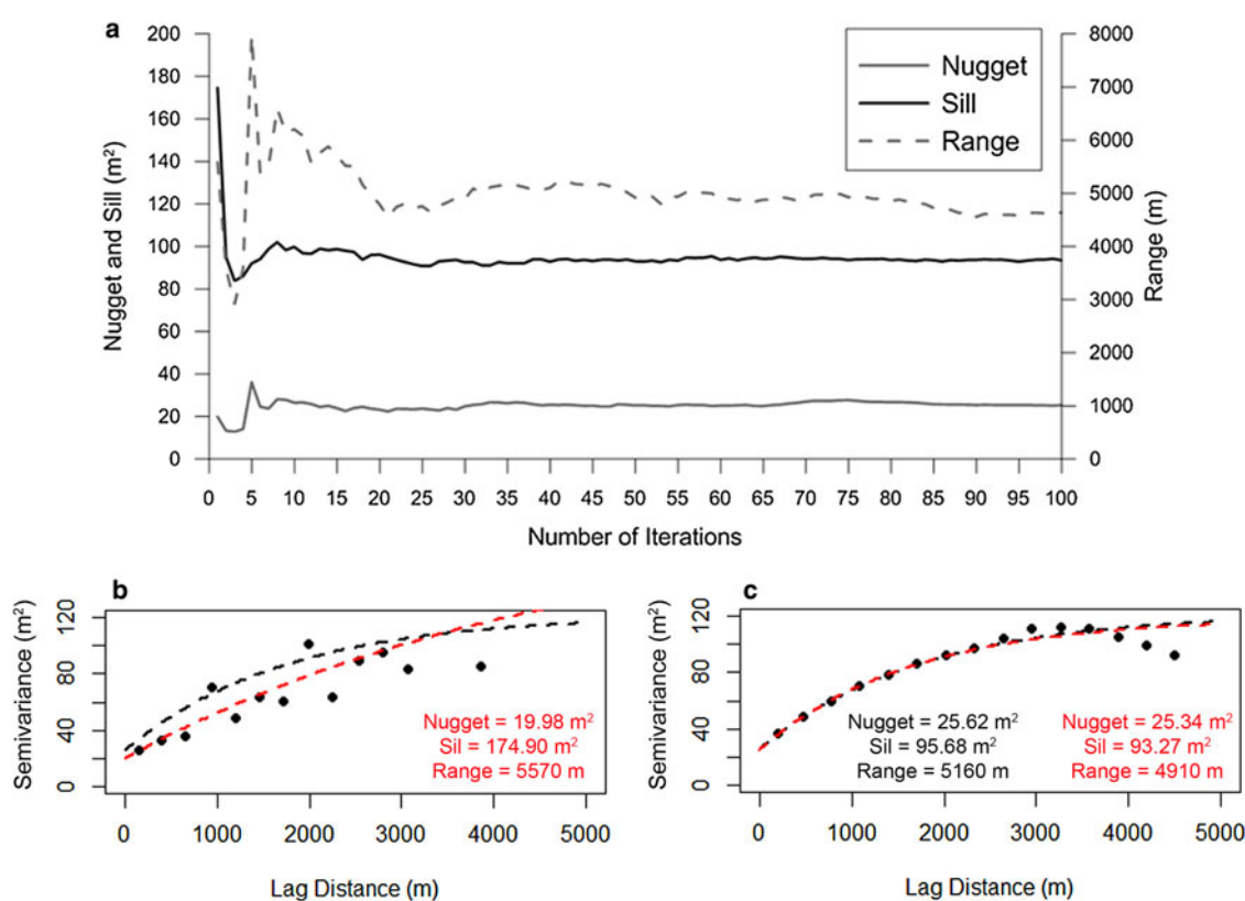
Fig. 13. (a) Stabilization of the parameters of the semi-variogram model as a function of the number of iterations of Mer the Glace; and Experimental semi-variogram (black circles) and fitted exponential model of Mer de Glace: the black dashed line stands for the full density topography and the red dashed line stands for the 1st iteration in (b) and for the 50th iteration in (c). The parameters of each semi-variogram model are included.
