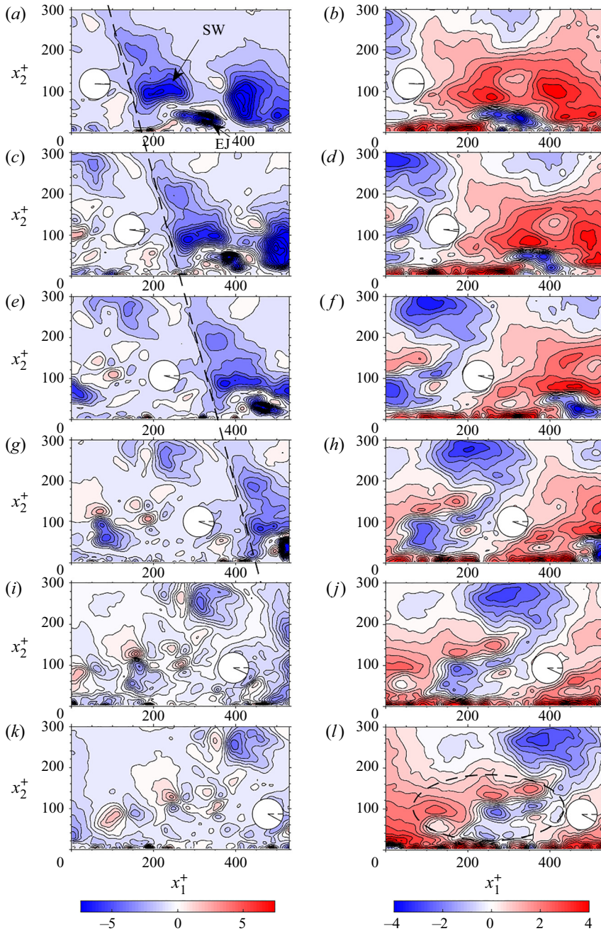
Figure 20. For S_4 , a sequence ( \Delta t^+ = 4.9 ) of equatorial wall-normal planes depicting the correlations of the instantaneous water fluctuating velocities (u_1 u_2)^+ (a,c,e,g,i,k), and the streamwise water fluctuating velocities u_1^+ (b,d,f,h,j,l). The hydrogel sphere is superposed as a filled white circle. Its initial orientation is indicated by a dashed line, while its changing orientation is indicated by a solid line. ‘SW’ and ‘EJ’ in (a) denote sweep and ejection motion, respectively. The slanted dashed line across (a,c,e,g) demarcates the upstream position of a sweep motion.
