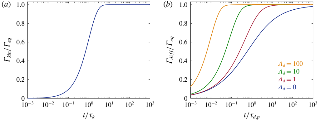
FIGURE 9. (a) Kinetically controlled adsorption (3.68) to an initially clean spherical surface. (b) Diffusion-controlled adsorption (3.71) to a spherical surface. Adsorption occurs over a faster time scale \tau_{d,s} in smaller bubbles ( \Lambda_d = L_d/R \gtrsim 1 ), and approaches equilibrium exponentially, rather than as 1/\sqrt{t} in the case of large bubbles ( \Lambda_d \rightarrow 0 ).
