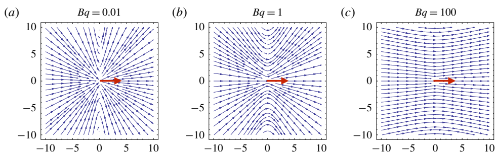
FIGURE 14. Streamlines of surface velocity as a result of a point force applied at the origin, following (3.108). Length is in units of R such that Bq = \eta_s/\eta R .
