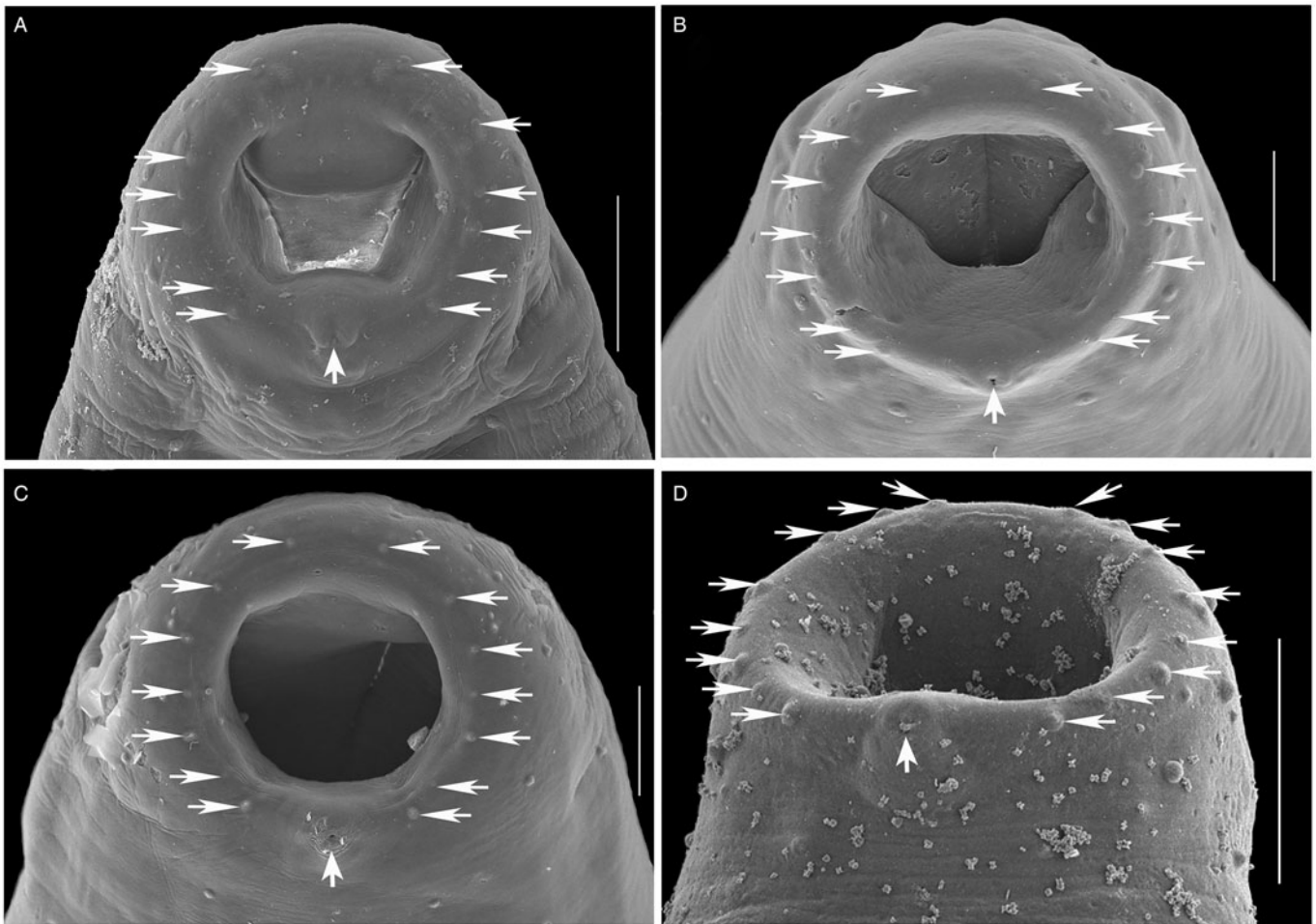
Figure 5. SEM photomicrographs of the oral sucker of 3 species of Schikhobalotrema showing the distribution of papillae: (A) Sch. minutum n. sp. ex St. notata , La Carbonera coastal lagoon, Yucatán, Mexico; (B) Sch. acutum ex T. acus , off Celestún, Yucatán, Mexico; (C) Sch. acutum ex T. pacificus , off Barra de Coyuca, Acapulco, Mexico and (D) Sch. acutum ex T. crocodilus , Lizard Island, Great Barrier Reef, Australia. Scale bars = 50 \mu m.
