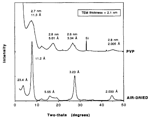
Figure 3. XRD patterns for sample DV4, normally a 45% expandable, R1-ordered I-S. Mean illite fundamental particle thicknesses measured for each 00 l reflection by the BWA technique for the upper, PVP-intercalated sample, are labeled in nm units. Peak positions are labeled in Å units. Si = a weak peak at d = 2.715 \text{ \AA} which is the Renninger double diffraction of (200) for the Si-metal substrate (according to Li and Albe 1993).
