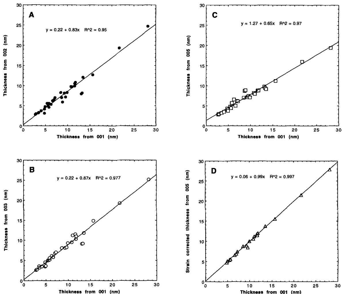
Figure 5. Extrapolated mean thicknesses measured for PVP-intercalated illites by the BWA technique for various 00l reflection orders (A, B, C) and for the strain corrected 005 (D, using lognormal-type illites) compared with thicknesses measured from the 001 reflection. Data from Table 1.
