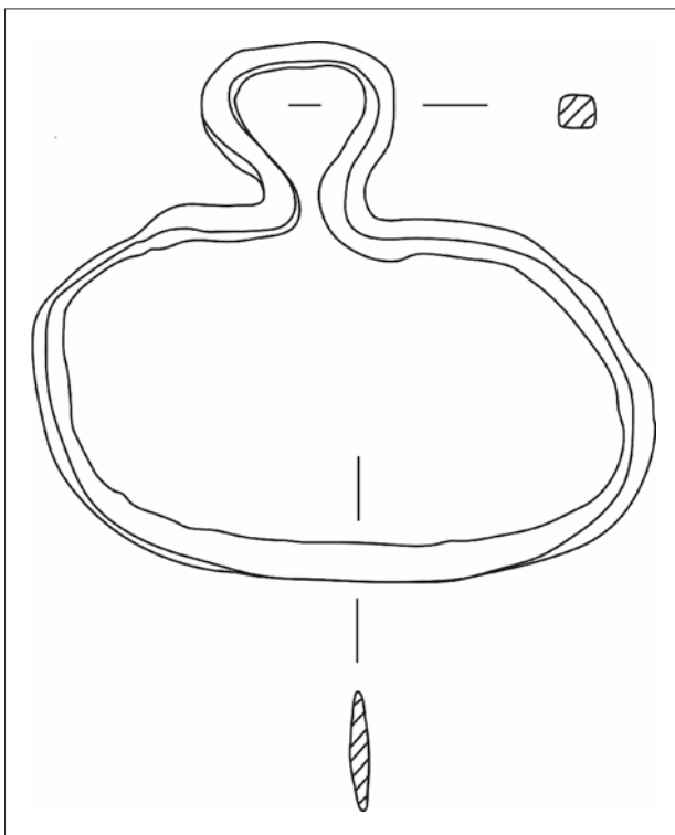
Fig. 5. Iron stirrup from Pergamum (redrawn after Gaitzsch 2005: Taf. 56, V29).
