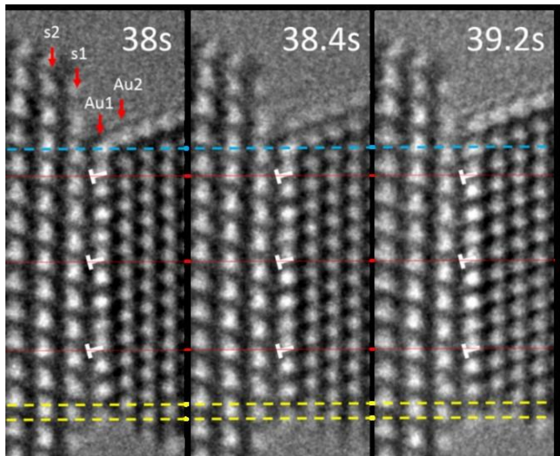
Figure 1. Rigid-body motion of a supported gold nanoparticle. The three red lines indicate the positions of dislocations. The interface layers are labeled s1 and Au1. The layer labeled Au2 is the second layer inside the Au particle counting from the interface, s2 is the second CeO 2 layer counting from the interface. The “T” symbol indicates the position of dislocations at the interface, where additional Au columns are present.
