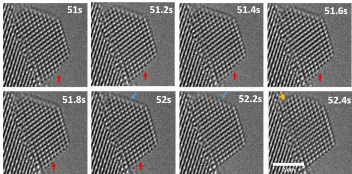
Figure 2. Red arrows indicate an atomic layer disappearing column-by-column on the (111) facet from 51s to 52s. Blue arrows indicate a newly formed layer on the (100) facet. At 52.2s, four columns appear at the blue arrow indicated on the (100) facet, two more columns are present in the next frame. Experimental conditions: room temperature, 4.5 Pa CO.
