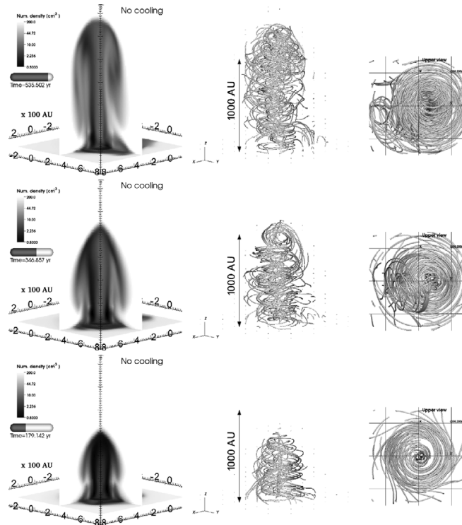
Figure 1. Evolution of the adiabatic magnetic tower. Left: logarithmic density grayscale maps. Middle: magnetic field lines. Right: field lines upper view. Time is the same row-wise. Open field lines are a visualization effect.
