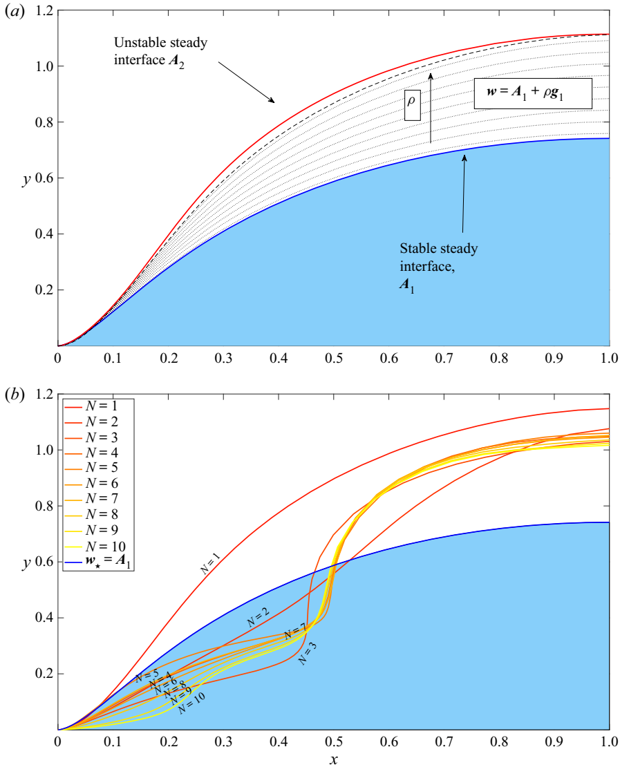
Figure 9. Perturbations of the advancing w_* = A_1 state. (a) ‘Stretch’ perturbations. The lower solid curve is the stable interface and the upper solid curve is the unstable interface. The dotted curves are different strength perturbations of the stable state according to (3.9) with i = 1 . The dashed curve corresponds to the perturbation which results in an identical value of Y as the A_2 state. (b) ‘Corrugation’ perturbations. The coloured curves are different strength perturbations of the stable state according to (3.10) for a fixed value of \rho and increasing N and the shaded region represents the nonlinear A_1 steady solution. Parameter values are Ca = 0.873 , \chi = 0.1 , \lambda = 0.1 .
