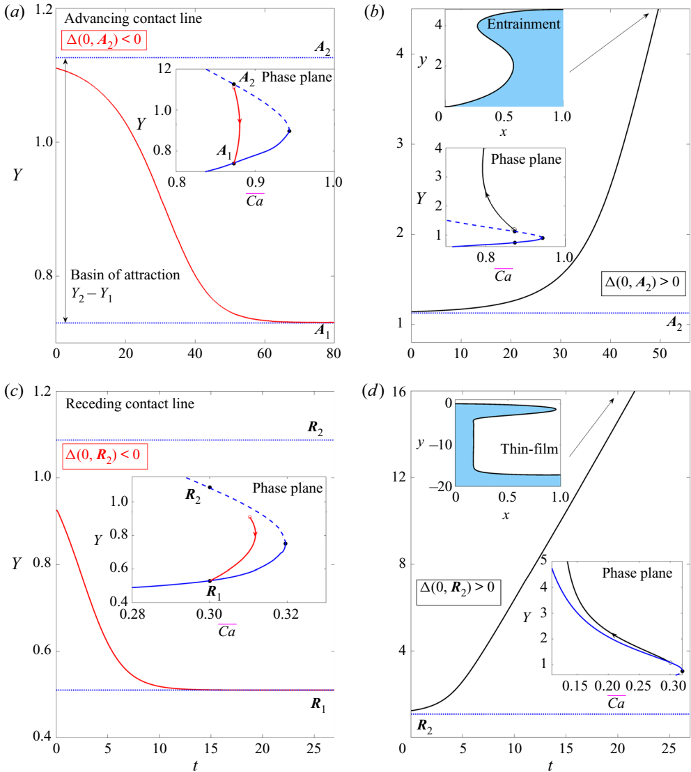
Figure 12. Time-dependent perturbations of the unstable branch using (4.3). (a,b) The advancing contact-line problem. (c,d) The receding contact-line problem. This figure shows perturbations from the solution labelled A_2/R_2 in figure 4. For both the advancing and receding contact line, when \Delta(0, A_2) < 0 the perturbation relaxes to the corresponding stable branch (a,c). When \Delta(0, A_2) > 0 the perturbation grows and in the case of the advancing contact line, entrainment occurs; see inset panel labelled ‘Entrainment’ in (b). For the receding contact line a thin film develops; see inset panel labelled ‘Thin-film’ in (d). The other inset panels show the phase plane in the (\overline{Ca}, Y) projection. The initial conditions are marked as open circles, the system trajectory is marked with arrows and the steady bifurcation is shown without arrows. The unstable branch can be considered as the basin boundary of attraction of the stable steady state. Parameter values are Ca = 0.873 , \chi = 0.1 , \lambda = 0.1 for the advancing problem and Ca = 0.3 , \chi = 0 , \lambda = 0.1 for the receding problem.
