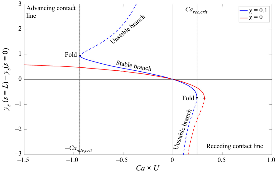
Figure 5. The advancing and receding steady solution curves for \lambda = 0.1 and \chi = 0 (red curves), \chi = 0.1 (blue curves). The horizontal axis is Ca scaled by U = \pm 1 and the vertical axis is y_s(s = L) - y_s(s = 0) , i.e. the signed version of Y . The critical Ca for each problem is denoted by a dotted line. The two problems are connected through the origin.
