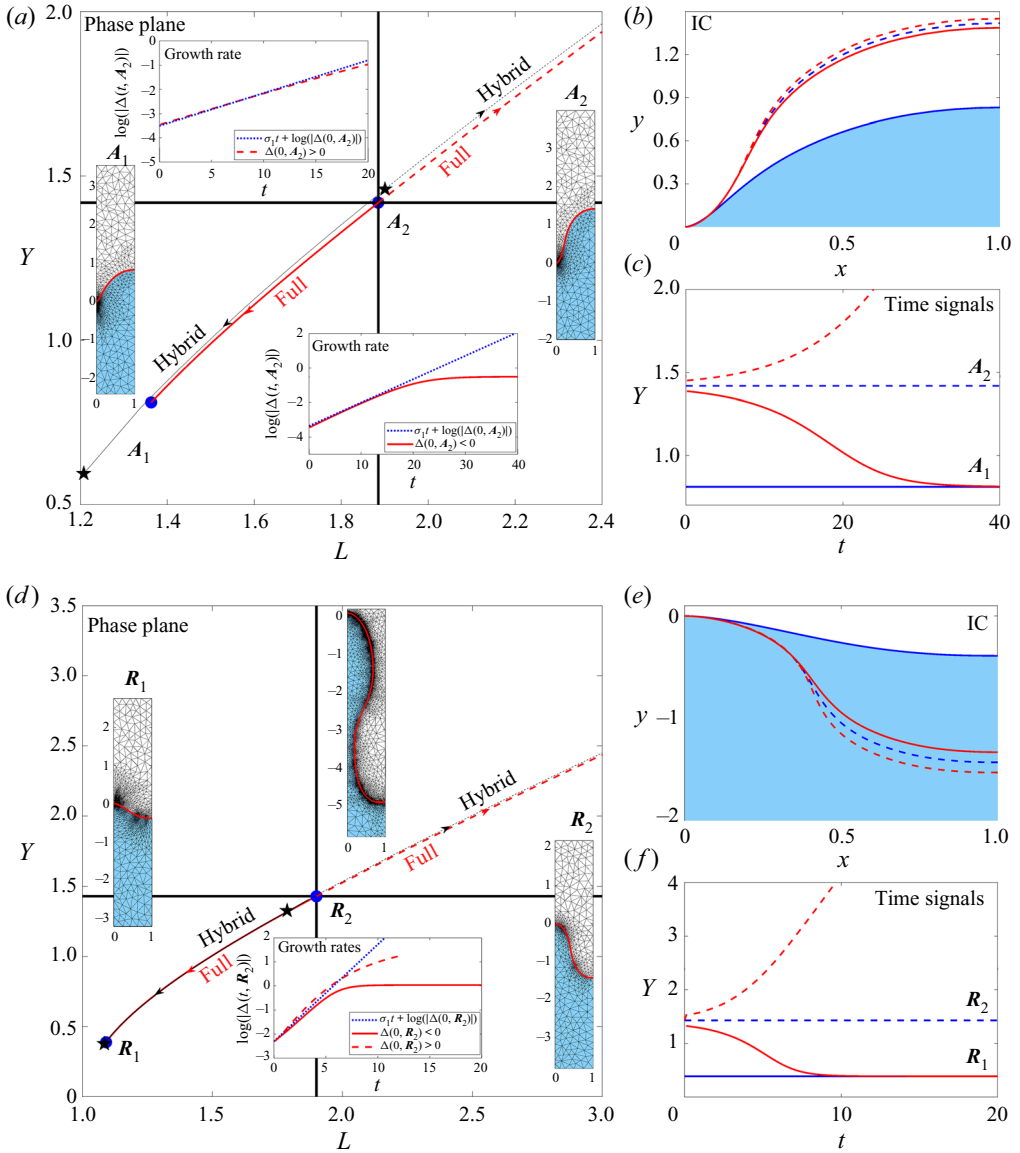
Figure 21. Time-dependent perturbations from the unstable state using the ‘stretch’ perturbations and the full two-layer model. (a–c) Advancing contact line. (d–f) Receding contact line. (a,d) The phase plane in the (L, Y) projection, with steady states indicated by circular markers (full model) and stars (hybrid model). Trajectories that result in a stable configuration ( \Delta(t = 0, A/R_2) < 0 ) are in solid lines and those that result in a transient behaviour ( \Delta(t = 0, A/R_2) > 0 ) are in dashed lines (red/full and black/hybrid). The inset diagrams show the two-layer mesh of the steady states with the interface as a solid red line, and comparisons of the growth rate of the simulations (solid/dashed red lines) and that predicted by the leading eigenvalue (dotted blue lines). In (d), the time-dependent state when air entrainment starts is also included. (b,e) The stable state (solid blue), unstable state (dashed blue) and the perturbations (solid/dashed red). (c,f) The time signals of each simulation. Parameter values are \chi = 0.1 , \lambda = 0.1 and Ca = 0.7 (advancing), Ca = 0.25 (receding).
