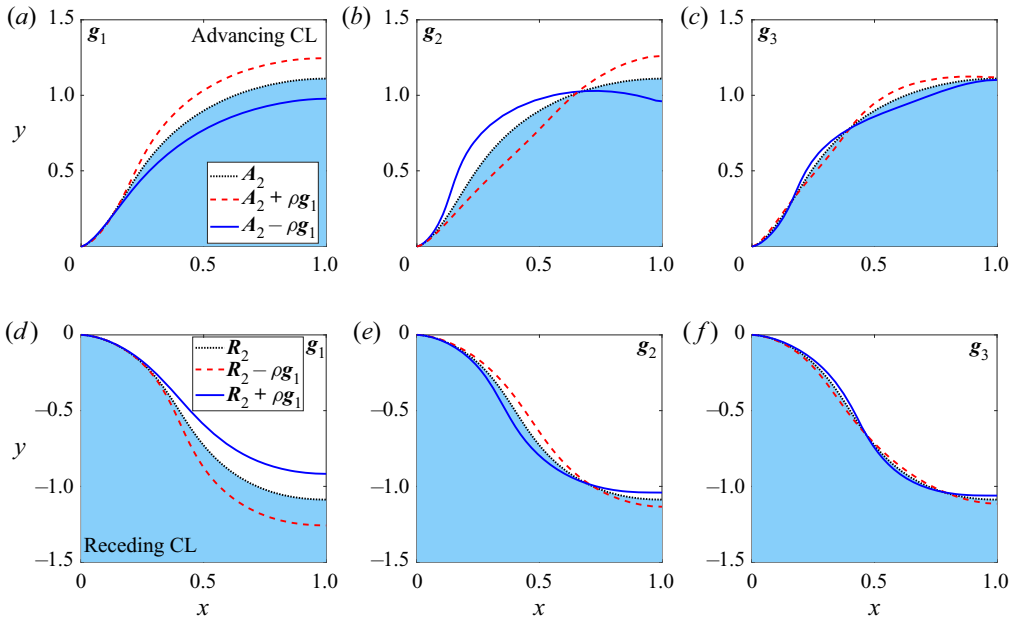
Figure 8. The eigenmodes of the unstable branch. The steady profile is shown as the dotted line. (a–c) The leading eigenmodes, g_1, g_2, g_3 , corresponding to the advancing w_* = A_2 ( Ca = 0.873, \chi = 0.1 ) solution in figure 4(a). (d–f) The leading eigenmodes corresponding to the receding w_* = R_2 ( Ca = 0.3, \chi = 0 ) solution in figure 4(b). In each case the eigenmodes cross the steady interface in successively more locations. The slip length is \lambda = 0.1 .
