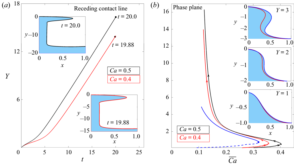
Figure 15. Time-dependent evolution for a receding contact line when Ca > Ca_{crit} and the system is at rest initially for \lambda = 0.1 , \chi = 0 . The different colour curves indicate different values of Ca = 0.4, 0.5 . (a) The time signal of Y with the final interface profiles in the inset. (b) The trajectories (curves with arrows) in the (\bar{Ca}, Y) phase-plane projection compared with the steady bifurcation curve (curve without arrows). The inset panels compare the interface profiles for the time-dependent evolution (red) and the steady solution branches (blue) at the same values of Y = 1, 2, 3 for the Ca = 0.4 case.
