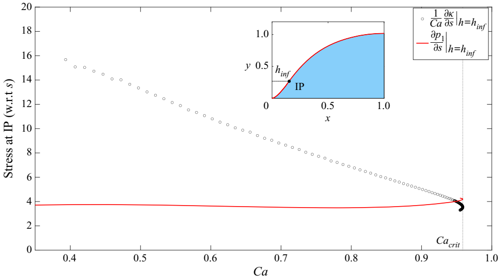
Figure 6. Comparison of the air-pressure gradient and the capillary-stress gradient for the steady solutions at the inflection point (IP) on the interface for the advancing contact-line problem. Parameter values are \chi = 0.1, \lambda = 0.1 .
