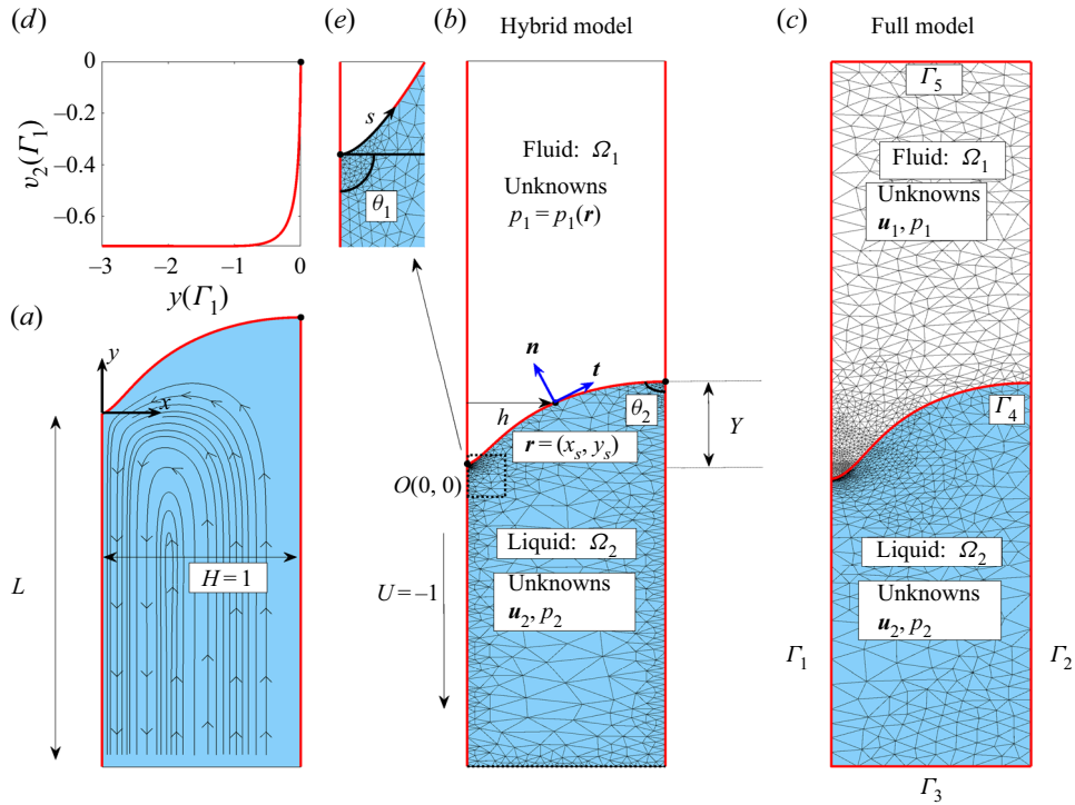
Figure 3. The computational domain for the hybrid and full models for an advancing contact line. The boundaries are denoted by \Gamma_i (labelled in c ) with the origin centred on the contact line. ( a ) A typical streamline pattern for a steady solution in the hybrid model. ( b ) The computational domain for the hybrid model. In this model we solve for the velocity and pressure in the liquid domain, but only solve for the pressure of the fluid on the interface boundary, \Gamma_4 . ( c ) The computational domain for the full model where the velocity and pressure fields are also solved in the fluid domain. ( d ) The vertical component of velocity along the moving plate, i.e. \Gamma_1 . ( e ) The enlargement near the contact line shows the mesh refinement required to ensure that the flow field is sufficiently resolved.
