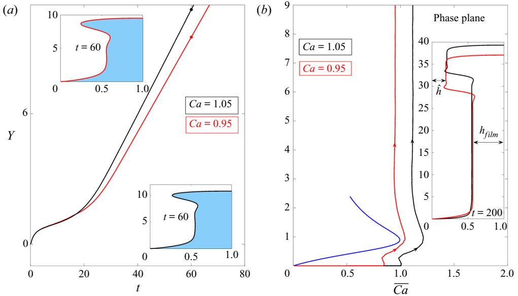
Figure 14. Time-dependent evolution for an advancing contact line when Ca > Ca_{crit} and the system is at rest initially for \lambda = 0.1 , \chi = 0.1 . The different colour curves indicate different values of Ca = 0.95, 1.05 . (a) The time signal of Y with interface profiles at the indicated times in the inset. (b) The trajectories (curves with arrows) in the (\overline{Ca}, Y) phase-plane projection compared with the steady bifurcation curve (curve without arrows). The inset compares the interface profiles for each Ca at t = 200 .
