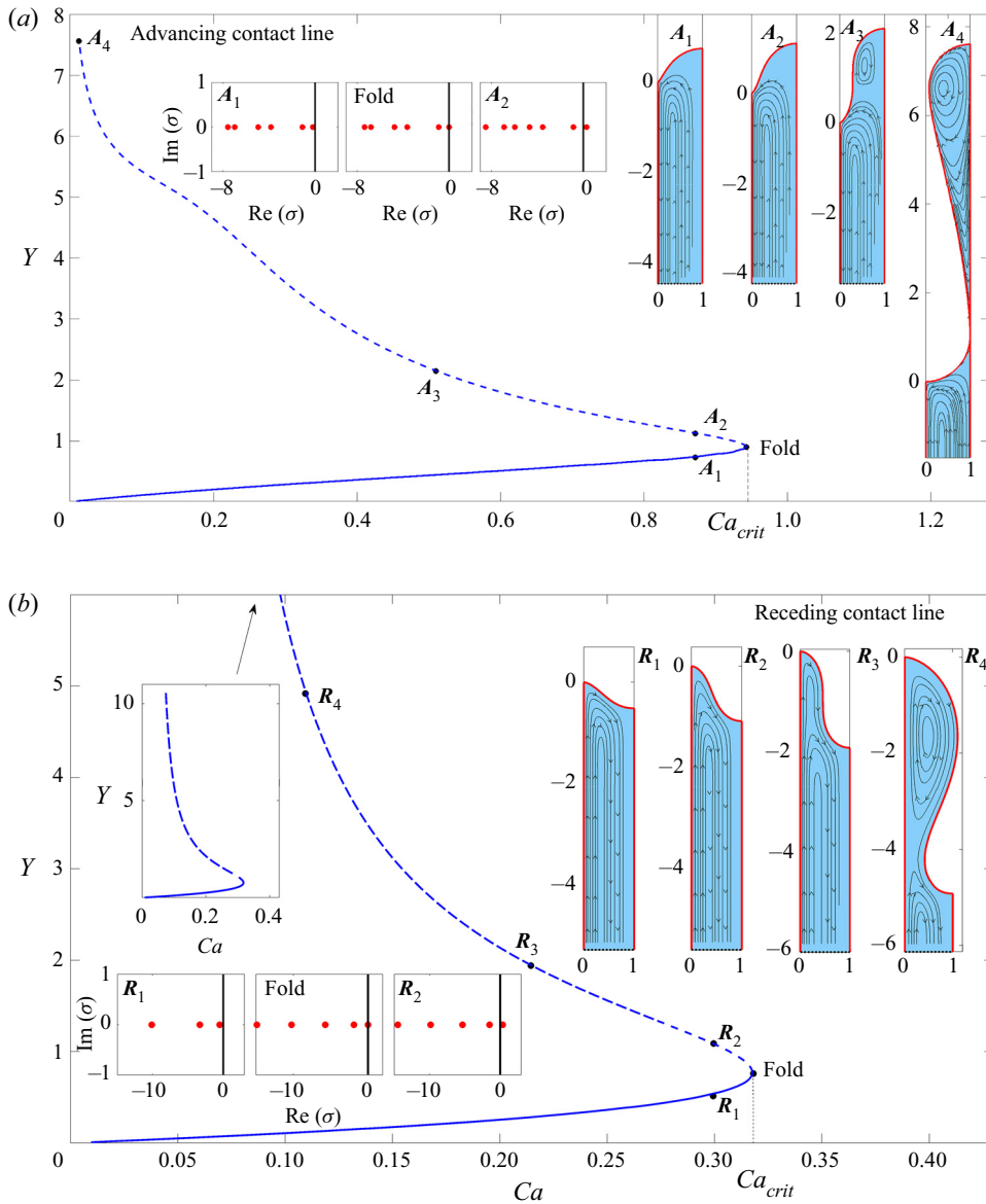
Figure 4. Solution curves for the advancing (a) and receding (b) contact lines. The values of the control parameters are \chi = 0.1 (a) and 0 (b) and \lambda = 0.1 for both panels. Individual solutions are labelled on the curve and correspond to the inset panels with the same label. The solid/dashed lines sections of the curve are the stable/unstable branches, respectively. The smaller insets show the eigenspectra for the A_1/R_1 and A_2/R_2 solutions and at the fold. Solutions A_3/R_3 are the solutions where the inflection point on the interface first becomes parallel to the plate, i.e. when dx_s/dy_s = 0 . In (a), A_4 is the solution just before the numerical calculations cease to converge. In (b), R_4 is the solution where the interface starts to ‘overhang’ the right plate. The top-left inset in (b) shows the bifurcation curve for larger Y .
