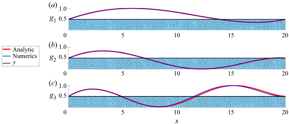
Figure 20. Comparison of eigenmodes, H/L = 40 , C = 3.0 . The different colour profiles indicate the analytic eigenmodes from (B2) and those obtained from the numerical calculations. (a) Eigenmode g_1 , corresponding to the largest eigenvalue; (b) g_2 and (c) g_3 are the eigenmodes for the next two largest eigenvalues.
