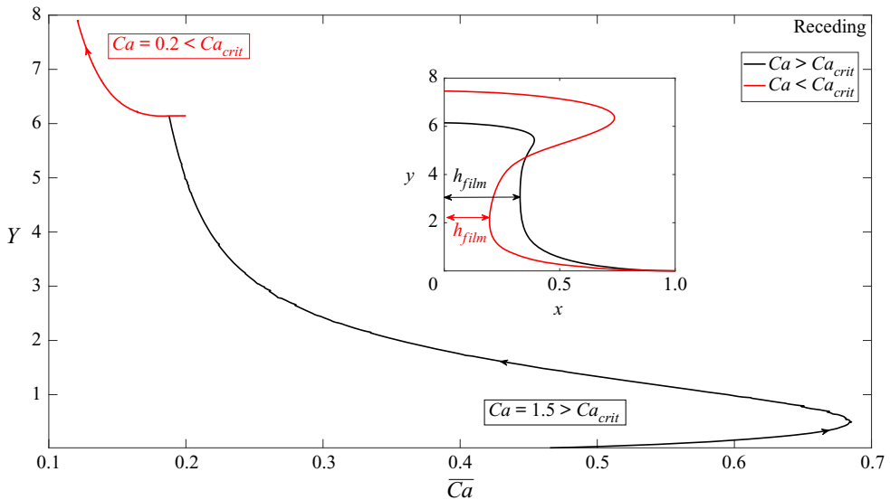
Figure 16. Time-dependent evolution for the receding contact line when Ca > Ca_{crit} and the system is at rest initially. Once a film has formed and Y = 6 , we set Ca < Ca_{crit} , as indicated in the figure by different colour trajectories and interface profiles. Other parameter values are \lambda = 0.1 , \chi = 0.0 .
