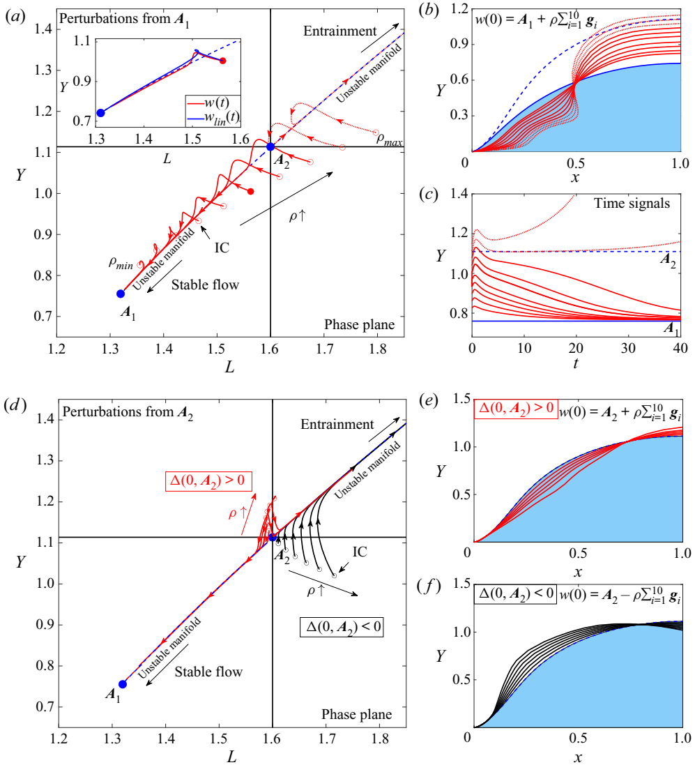
Figure 13. Time-dependent perturbations using the ‘corrugation’ perturbations. Perturbations from the solutions labelled in figure 4(a) using (4.6). (a–c) Perturbations from A_1 . (d–f) Perturbations from A_2 . (a, d) Time-dependent trajectories in the in the (L, Y) phase-plane projection. Initial perturbations (IC) are denoted by open circles and steady states by large solid circles. The dashed blue lines indicate the unstable manifold of the A_2 state and the solid black lines are artificial axes centred on the unstable A_2 state. (a) Each red curve indicates a time-dependent trajectory with a different value of increasing \rho , as indicated by the black arrow, the initial conditions with minimum and maximum \rho have been labelled. The solid trajectories correspond to initial perturbations that return to the steady state and dotted trajectories correspond to trajectories that result in entrainment. The inset shows the linear response given in (3.6) for a particular initial condition marked with a filled circle in the main panel. (b) The initial interfaces of the trajectories shown in (a) are shown as solid lines and the A_1 and A_2 steady states are shown using the shaded area and a dashed line, respectively. (c) The corresponding time signals of Y for the trajectories shown in (a). (d) Red/black curves indicate trajectories with initial conditions \Delta(0, A_2) positive/negative, respectively. (e, f) The initial conditions corresponding to the trajectories in (d) with the unstable state indicated by the shaded area. Parameter values are Ca = 0.873 , \chi = 0.1 , \lambda = 0.1 .
