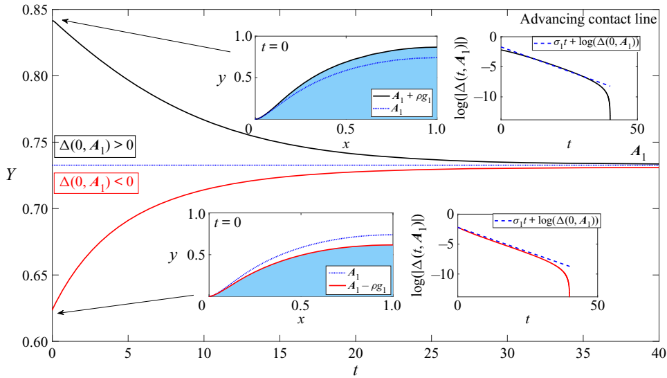
Figure 11. Time-dependent perturbations of the advancing contact line using (4.3). This figure shows perturbations from the solution labelled A_1 in figure 4(a). The two different initial conditions are shown in the inset panels corresponding to the same colour lines in the main panel. Whether \Delta(0, A_1) > 0 or \Delta(0, A_1) < 0 the system relaxes back to the stable state. The inset panels on the right show the time signal of \log(|\Delta(t, A_1)|) as compared to the predicted growth rate \sigma_1 . Parameter values are Ca = 0.873 , \chi = 0.1 , \lambda = 0.1 .
