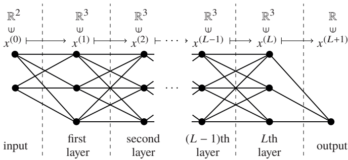
Figure 2.1. The graph associated to the outputs \Upsilon^{3,L}(\sigma; 2, 1) of a fully connected network with input dimension 2, width 3, L hidden layers and output dimension 1.
