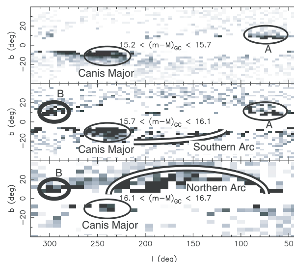
Figure 1 Binned M-giant counts about the Galactic plane. The three panels denote different magnitude (and hence distance) ranges, with the galactocentric distance modulus labelled upon each panel. Also in each panel, the counts represent the asymmetry between the north and south (i.e. southern data subtracted from the north, and vice versa). The main body of Canis Major and prominent structures in the M-giant distribution are noted (fig. 5 from Martin et al. 2004).
