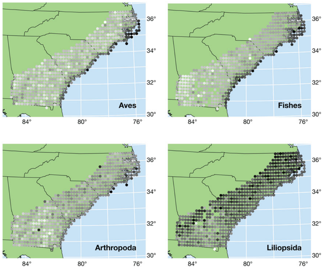
Figure 5. Representative maps of nonmetric multidimensional scaling (NMS) axis 1 scores for the 0.2° grid cells. Relative NMS scores are indicated with grayscale, from black (most negative score) to white (most positive score). Maps for all taxa are included in the Supplementary Material.
