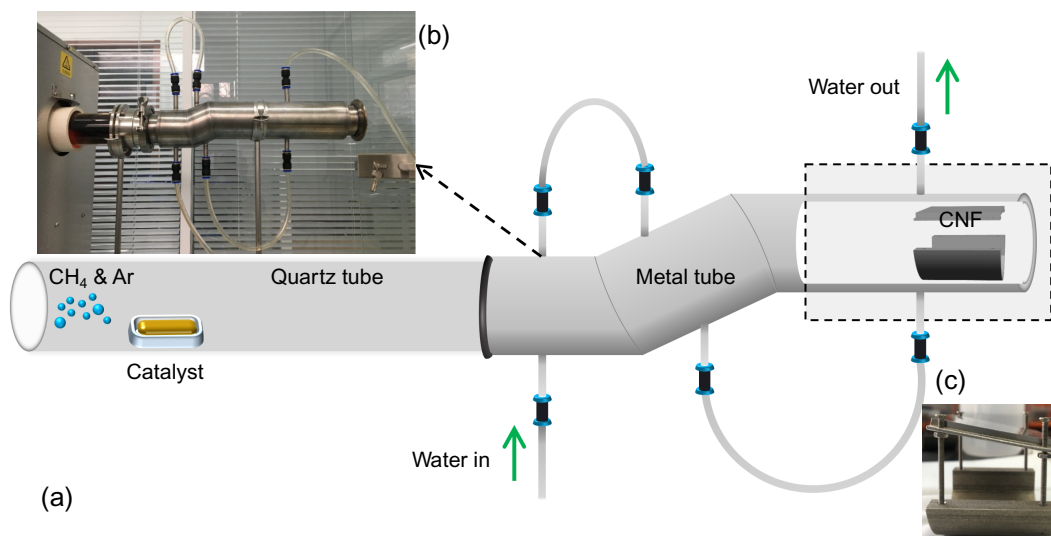
Figure 1. (a) Setup of an FCCVD system equipped with the water-cooling component. (b) A photo of the water-cooling component. (c) Target frame used to fix the target holder or the Si wafer in the deposition zone.
