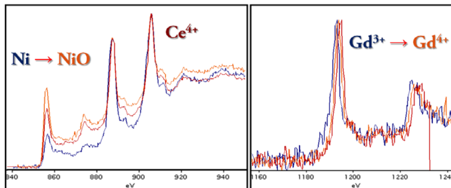
Figure 1. Electron energy loss spectra from GDC-Ni interface from Ni-L, Ce-M, and Gd-M edges at R.T. (blue), 200 (orange), and 400°C (red).
