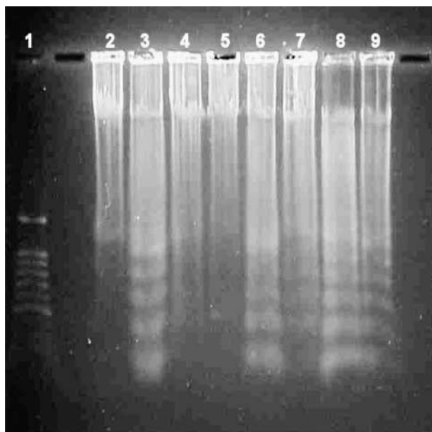
Fig. 1. Induction of DNA fragmentation following incubation for 24 h with 30 \mu\text{M} 7 \beta -hydroxycholesterol (7 \beta -OH chol) or 120 \mu\text{M} \alpha -epoxysterol ( \alpha -epox), \beta -epoxysterol ( \beta -epox), \alpha -epoxysterol- \beta -epoxysterol (6:1) mixture ( \alpha/\beta -epox), triolsterol (triol), 7-ketosterol (7-keto) or 7 \beta -hydroxysterol (7 \beta -OH). DNA fragmentation was assessed by agarose gel electrophoresis. Lane 1, molecular weight marker; lane 2, solvent control; lane 3, 7 \beta -OH chol; lane 4, \alpha -epox; lane 5, \beta -epox; lane 6, \alpha/\beta -epox; lane 7, triol; lane 8, 7-keto; lane 9, 7 \beta -OH.
