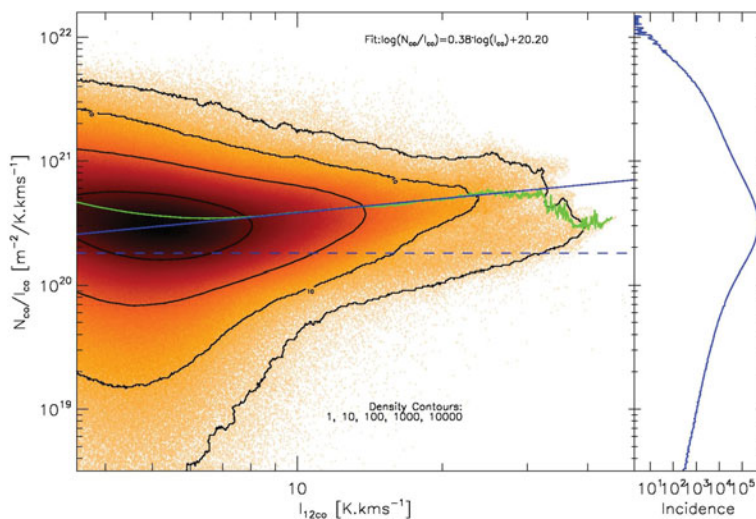
Figure 1. Ratio of CO column density N to integrated intensity I , from ThrUMMS (Barnes et al. (2015)).
