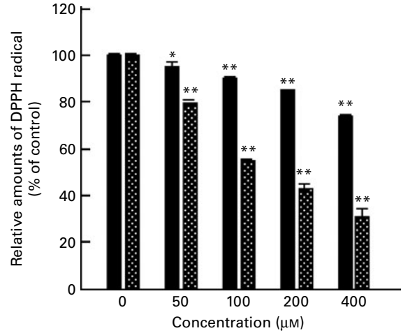
Fig. 5. Free radical-scavenging activity of butylated hydroxytoluene (BHT; ■) and quercetin (▨). The relative amount of free radicals generated by 1,1-diphenyl-2-picrylhydrazyl (DPPH) was determined as described in the Materials and methods. The amount of free radicals generated by DPPH was set at 100% and the relative amount of each free radical after treatment with BHT and quercetin was evaluated. Values are means ( n 3), with standard deviations represented by vertical bars. Mean value was significantly lower than that of the untreated control: * P <0.05, ** P <0.01.
