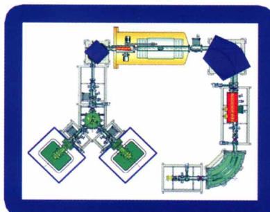
Multi Ion Source Compact Carbon AMS
