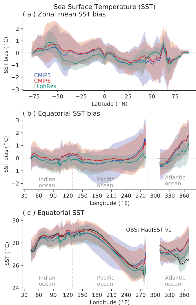
Figure 3.24 | Biases in zonal mean and equatorial sea surface temperature (SST) in CMIP5 and CMIP6 models. CMIP6 (red), CMIP5 (blue) and HighResMIP (green) multi-model mean (a) zonally averaged SST bias; (b) equatorial SST bias; and (c) equatorial SST compared to observed mean SST (black line) for 1979–1999. The inter-model 5th and 95th percentiles are depicted by the respective shaded range. Model climatologies are derived from the 1979–1999 mean of the historical simulations, using one simulation per model. The Hadley Centre Sea Ice and Sea Surface Temperature version 1 (HadISST) (Rayner et al., 2003) observational climatology for 1979–1999 is used as the reference for the error calculation in (a) and (b); and for observations in (c). Further details on data sources and processing are available in the chapter data table (Table 3.SM.1).
