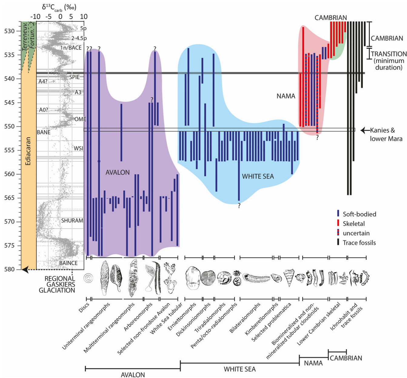
Figure 7. (Colour online) Compilation of ranges of known major Ediacaran to earliest Cambrian macrofossils (soft-bodied and skeletal) and major trace fossil groups (ca. 580–528 Ma) calibrated to radiometric dates and an updated composite \delta^{13}\text{C} curve (after Yang et al. 2021; Bowyer et al. 2022, 2023a, 2023b; Nelson et al. 2023). Figure shows the possible age of the Kanies and lower Mara Members based on the most parsimonious global radiometric, chemostratigraphic and preliminary biostratigraphic considerations. Proposed re-division of Avalon, White Sea and Nama assemblages is shown, based on morphogroup membership alone, with the appearance of the transitional and Cambrian assemblage from ca. 535 to 536 Ma. Question marks denote uncertainty in the precise age of specific formations/members (see Supplementary Information of Bowyer et al. 2023b).
