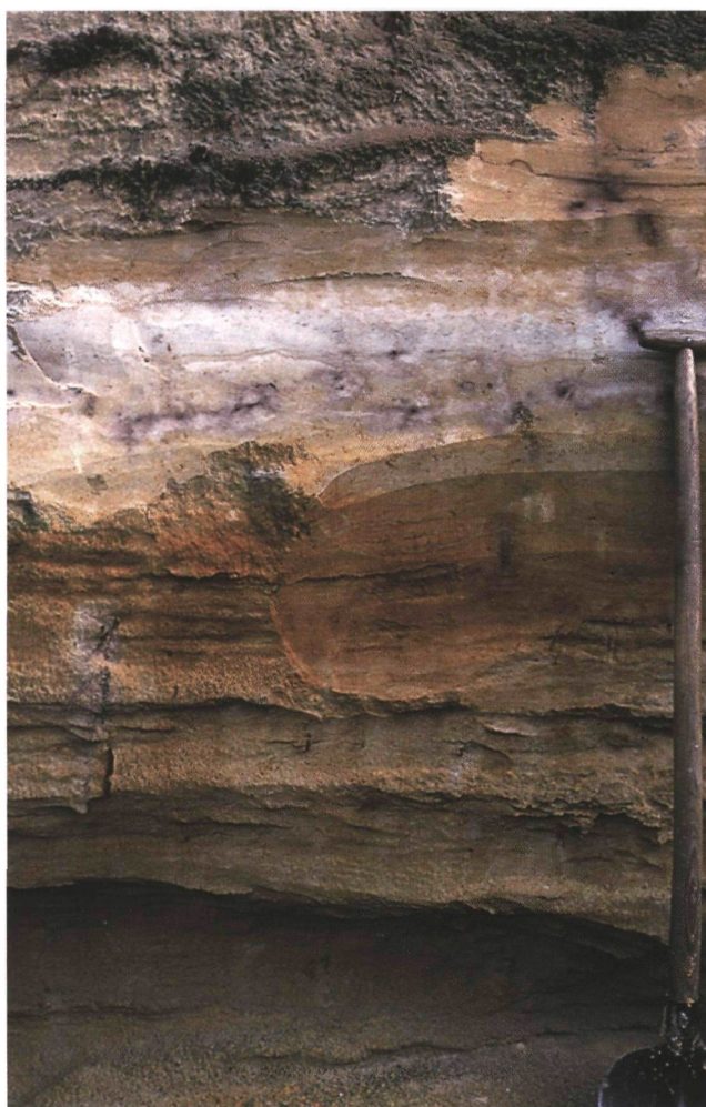
Fig. 1. Usselo soil in Weelde, Belgium (photo C. Kasse).
