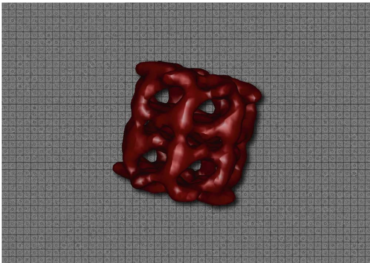
Fig. 1. Leginon was used to acquire over 100,000 GroEL particles in less than 24 hours. Shown are some of particles and a preliminary electron density map.
