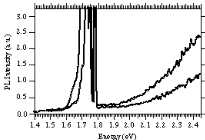
Figure 4. 5 K PL of bare sapphire and undoped GaN on a sapphire substrate, excited by 2.95 eV light. It is clear that the bare sapphire sample has luminescence in the 2.1 to 2.5 eV range. The chromium emission from the sapphire is visible in both spectra between 1.6 and 1.8 eV.
