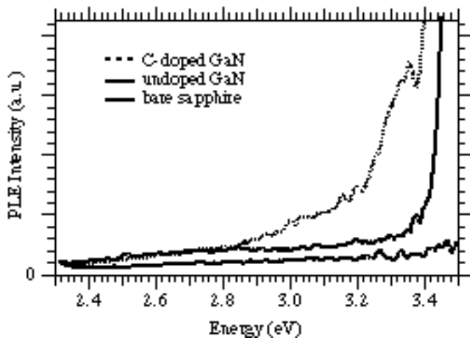
Figure 2. 5 K PLE spectra, detected at 2.2 eV, of C-doped GaN (top spectrum), undoped GaN (middle), and bare sapphire (bottom), each spectrum taken under identical conditions and corrected for the intensity spectrum of exciting light.
