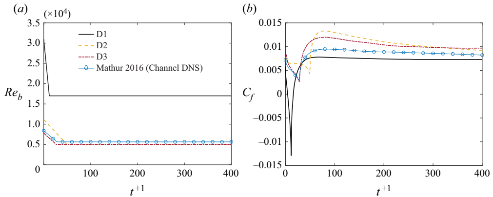
Figure 1. (a) Ramp-down change in the bulk Reynolds number Re_b for the present cases D1 (—), D2 (---) and D3 (- · - · -). Case D3 is compared with the channel flow DNS by Mathur (2016) (○). (b) Transient response of the skin friction coefficient for the cases depicted in (a).
