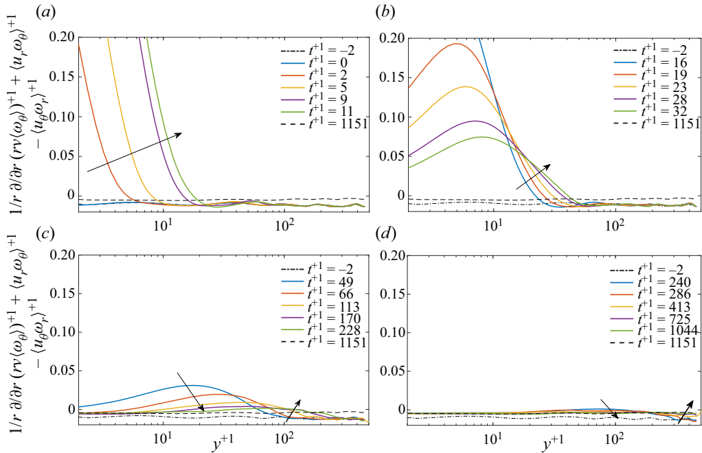
Figure 14. Time evolution of the mean vorticity flux 1/r\partial/\partial r (rv\langle\omega_\theta\rangle)^{+1}/\partial r^{+1} + \langle u_r\omega_\theta\rangle^{+1} - \langle u_\theta\omega_r\rangle^{+1} throughout the four transitional stages underwent by a rapidly decelerating flow: (a) inertial, (b) friction recovery, (c) turbulence decay and (d) core relaxation.
