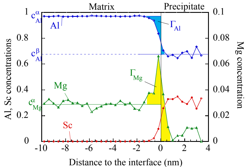
Fig. 2: Proximity histogram for a \text{Al}_3\text{Sc} precipitate obtained after aging at 300^\circ\text{C} for 1040 hours.
