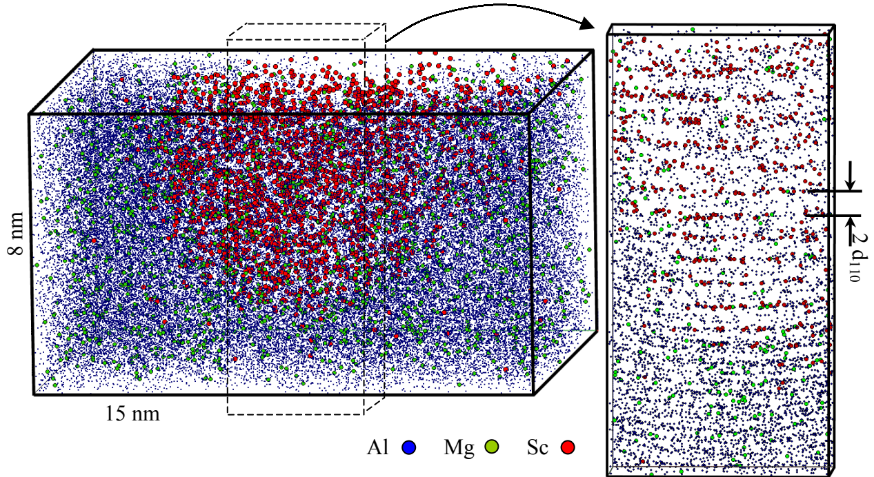
Fig. 1: (a) 3D reconstruction of an \text{Al}_3\text{Sc} precipitate analysed after aging at 300^\circ\text{C} for 1040 hours (b) Slice showing the [110] planes.
