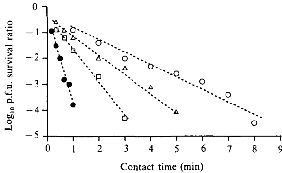
Fig. 2. Inactivation kinetics of poliovirus 1 at pH 7.0, 25 °C. Free available chlorine and cyanuric acid concentrations were 0.5 mg/l and 0 mg/l (●), 0.5 mg/l and 30 mg/l (○), 1.0 mg/l and 30 mg/l (△), and 1.5 mg/l and 30 mg/l (□), respectively. ---, Regression line.
