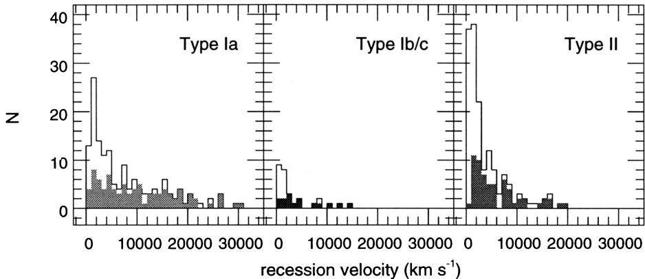
Figure 2. Histograms of the distribution of supernovae in distance bins. The shaded areas are statistics starting only 1989. The bin width is 1000 \text{ km s}^{-1} . Thus only the two closest bins are likely to be sensitive to peculiar galaxy motions.
