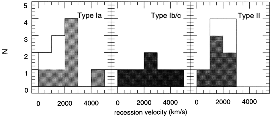
Figure 3. Same as Fig. 2 for the supernovae of Muller et al. (1992), shaded area, and the sample including the supernovae discovered during the first year of LOSS (Treffers et al. 1994).
