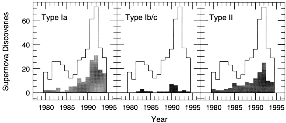
Figure 1. Supernova discoveries between 1980 and 1994. The data and classifications are from the Asiago Supernova Catalog (Barbon et al. 1989) for all supernovae before 1989 and according to IAU Circulars and the literature thereafter. The line histogram shows the total number of supernovae discovered per calendar year and the shaded areas the supernovae of the particular type.
