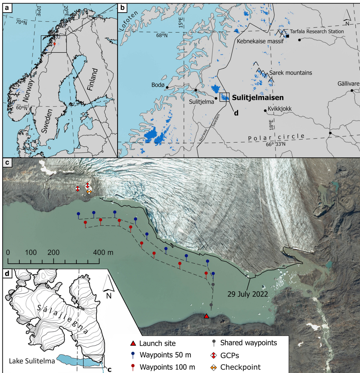
Figure 1. (a) and (b) Location of Sulitjelmaisen and Sálajiegna in northern Scandinavia. Glacier areas (blue) are retrieved from the GLIMS database (GLIMS Consortium, 2005). (c) Sálajiegna's glacier front seen on the 0.4 m aerial RGB image by © Lantmäteriet, the Land Survey of Sweden, 24 August 2022. Waypoints for the USV photogrammetric survey along the calving front are indicated with red and blue markers. The black solid line marks the calving front position as of 29 July 2022. (d) Sálajiegna's outline based on Copernicus Sentinel 2 imagery from 4 September 2022, processed by ESA, and legend for (c).
