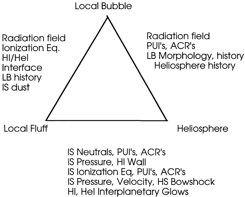
Fig. 1. This figure shows the links between the physics of the Local Bubble, Local Fluff, and Heliosphere. Abbreviations in the figure and text are: CSSS=cloud surrounding the solar system; LFC=Local Fluff complex; ISM=interstellar matter; LISM=local ISM; PUI=pick-up ions; IS=interstellar; IE=ionization equilibrium; ACR=anomalous cosmic rays; LB=Local Bubble; HS=heliosphere; SXRb=soft X-ray background; SCA=Scorpius-Centaurus Association.
