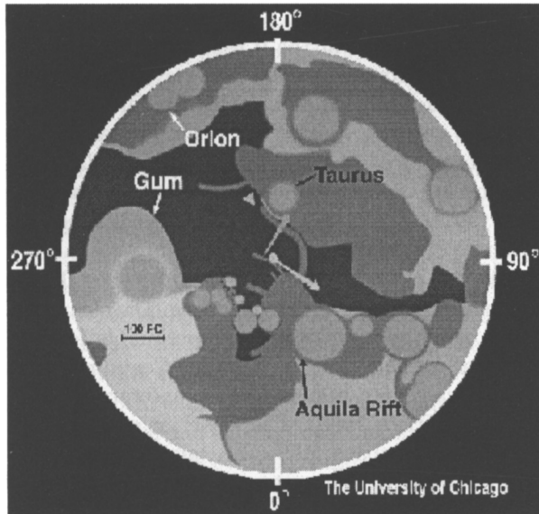
Fig. 2. The distribution of interstellar molecular clouds (traced by the CO 1->0 115 GHz rotational transition, Dame and Thaddeus 1985) and diffuse gas (traced by E(B-V) color excess due to the reddening of starlight by interstellar dust Lucke 1978) within 500 pc of the Sun are shown. The round circles are molecular clouds, and the shaded material is diffuse gas. Interstellar matter is shown projected onto the galactic plane, and the plot is labeled with galactic longitudes. The distribution of nearby interstellar matter is associated with the local galactic feature known as “Gould’s Belt”, which is tilted by about 15–20° with respect to the galactic plane. Thus, the ISM towards Orion is over 15° below the plane, while the Scorpius-Centaurus material (longitudes 300°–0°) is about 15–20° above the plane. Also illustrated are the space motions of the Sun and local interstellar gas, which are nearly perpendicular in the LSR velocity frame. The three asterisks are three subgroups of the Scorpius-Centaurus Association. The three-sided star is the Geminga Pulsar. The arc towards Orion represents the Orion’s Cloak supernova remnant shell. The other arcs are illustrative of superbubble shells from star formation in the Scorpius-Centaurus Association subgroups. The smallest (i.e. greatest curvature) shell feature represents the Loop I supernova remnant.
