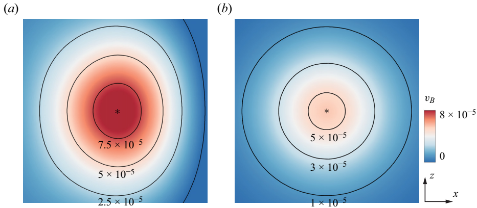
Figure 14. Contour of (a) v_B in the DNS and (b) v_B^{br} from the model in (4.27) in Case 1 in the x - z plane at y^+ = 1 and at t = 1 in Case 1. The asterisk marks the position of vortex bursting projected on the x - z plane.
