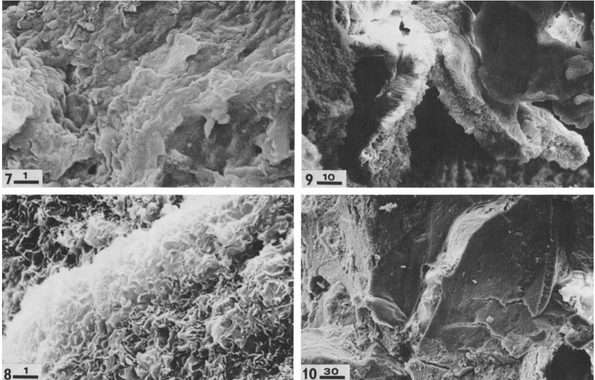
Figure 7. Scanning electron micrograph of ultrafine, dense aggregate of montmorillonite filling space of original hyaloclasts. Rokle bentonite, Czechoslovakia. Bar = 1 \mu\text{m} .
