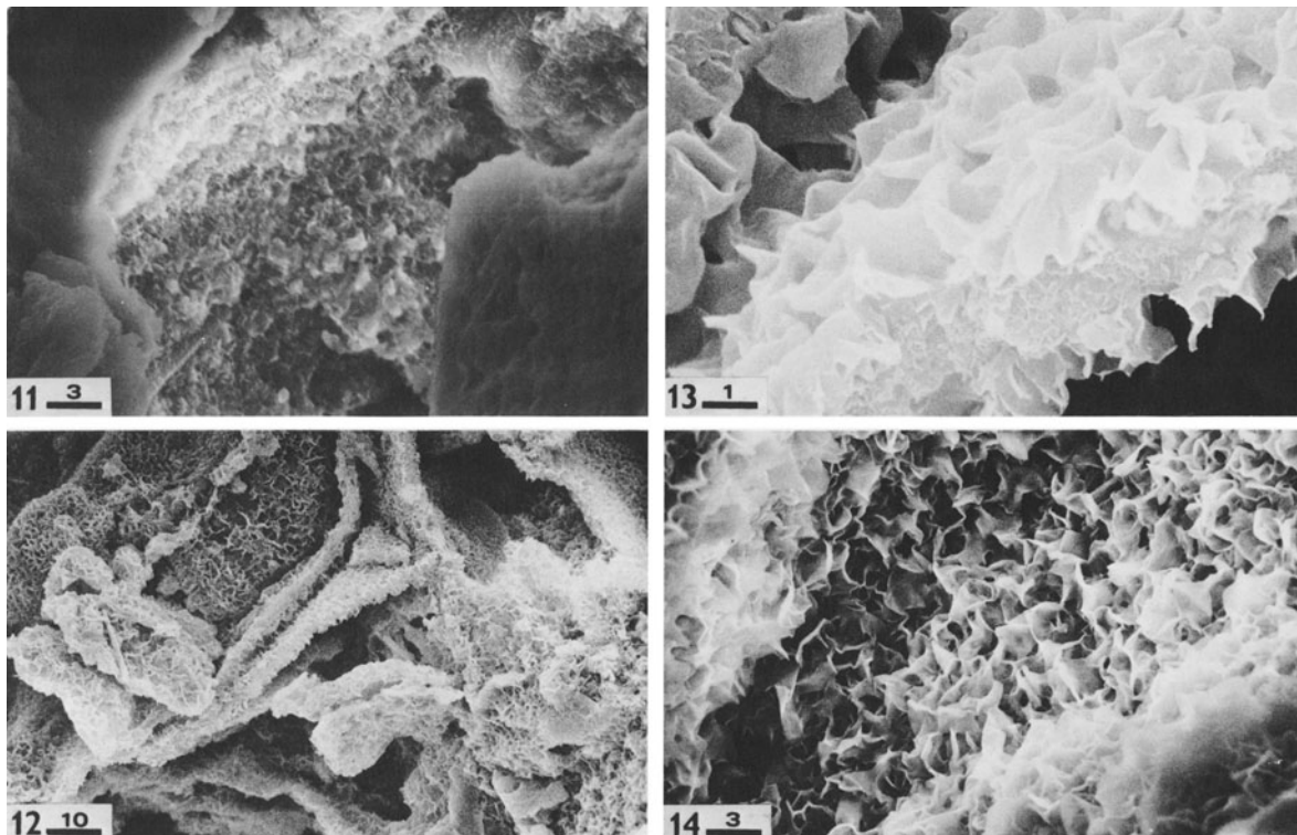
Figure 11. Imperfect but coarse honeycomb texture of montmorillonite aggregate filling crack. Rokle bentonite, Czechoslovakia. Bar = 3 \mu\text{m} .
