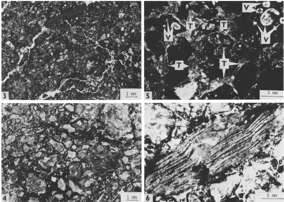
Figure 3. Photomicrograph of thin section of original shapes of fine-grained arenite hyaloclasts transformed into montmorillonite, Rokle bentonite deposit, Czechoslovakia; uncrossed nicols, 12 \times . Note one black-gray biotite in top center.
