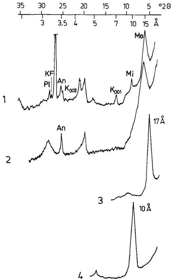
Figure 15. X-ray powder diffractograms of (1) the olive gray, raw bentonite, unoriented preparation, and of its <1\text{-}\mu\text{m} size fraction as oriented preparation, in (2) natural, (3) glycolated state, and (4) heated at 550^\circ\text{C} for 2 hr.
