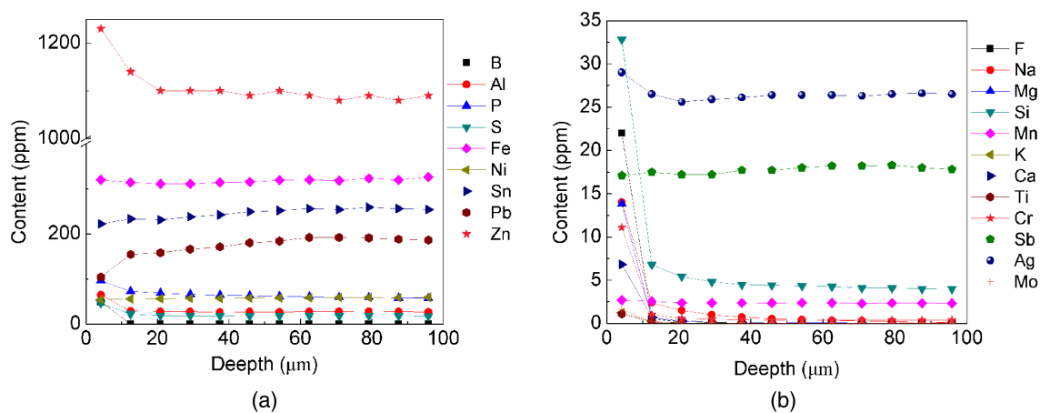
Figure 6. The trace elements distribution of a copper part. (a) Surface content >50 ppm. (b) Surface content <50 ppm.
