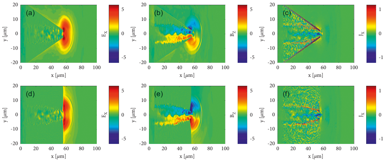
FIGURE 2: Snapshots of the time-averaged electric field E_x ((a), (d)) normalized by m_e \omega_0 c / e , the z-component of magnetic field B_z , ((b), (e)) normalized by m_e \omega_0 / e and currents in x-axis direction J_x , and ((c), (f)) normalized by ec n_c at t = 85T_0 for the conical target (top) and the uniform rectangle target (bottom).
