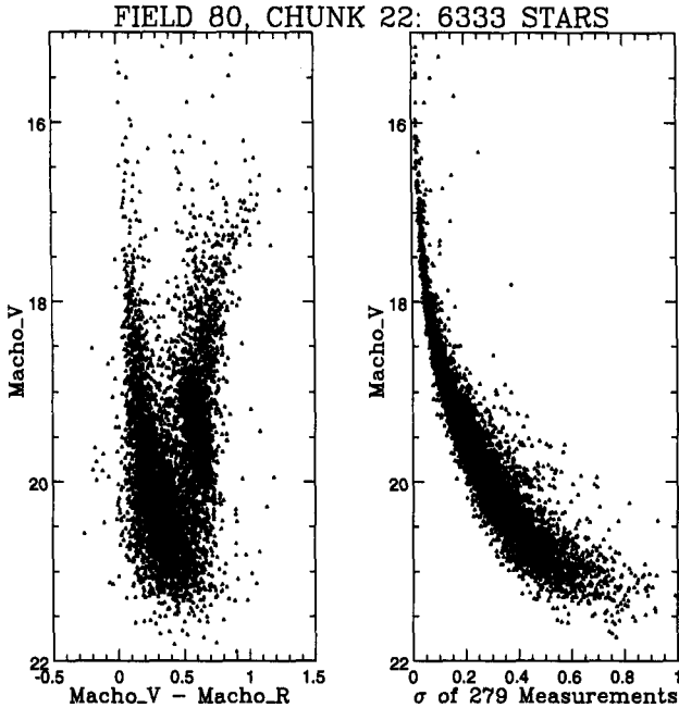
Figure 1. The left panel is a colour magnitude diagram prepared from the median of 279 measurements of the stars in a 3 \times 3 arcmin region of the LMC bar. The right panel plots the standard deviation of the time series used to calculate the median MACHO_V magnitude.
