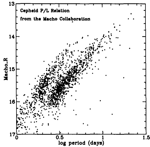
Figure 3. P/L relation for 1540 Cepheids from the first year's analysis of MACHO data.
