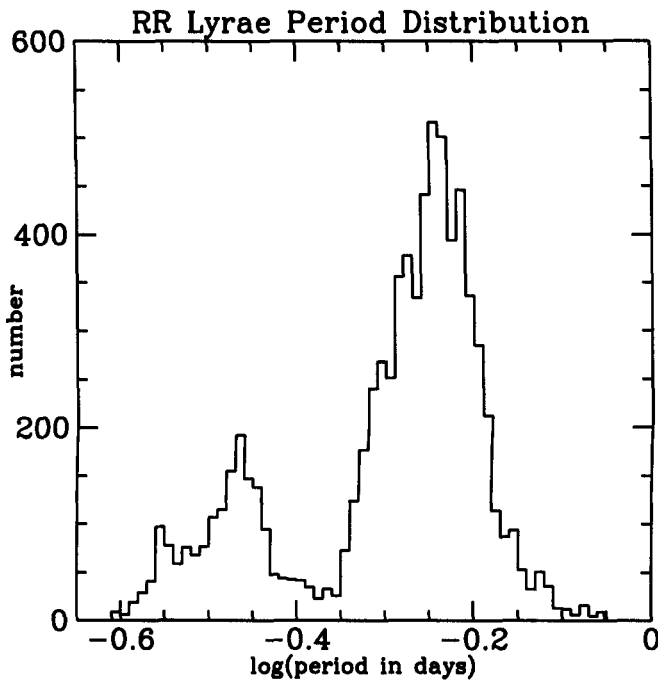
Figure 4. Histogram of periods found for 7652 RR Lyrae in the central 10.5 square degrees of the LMC.
