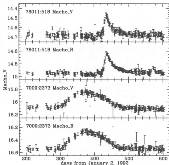
Figure 5. Light curves demonstrating the two general types of outbursts observed in the bumpers.
