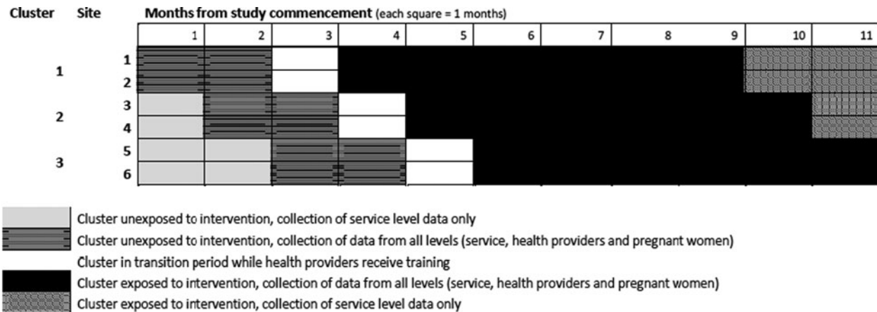
Fig. 2. Schema of Step-Wedge Cluster Randomised Design for ICAN QUIT in Pregnancy (reproduced with permissions from authors) (Bar-Zeev et al. , 2017).
