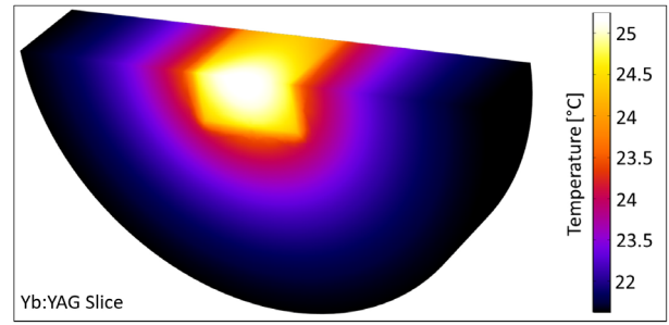
Figure 2. A slice through the pumped Yb:YAG model in COMSOL.
