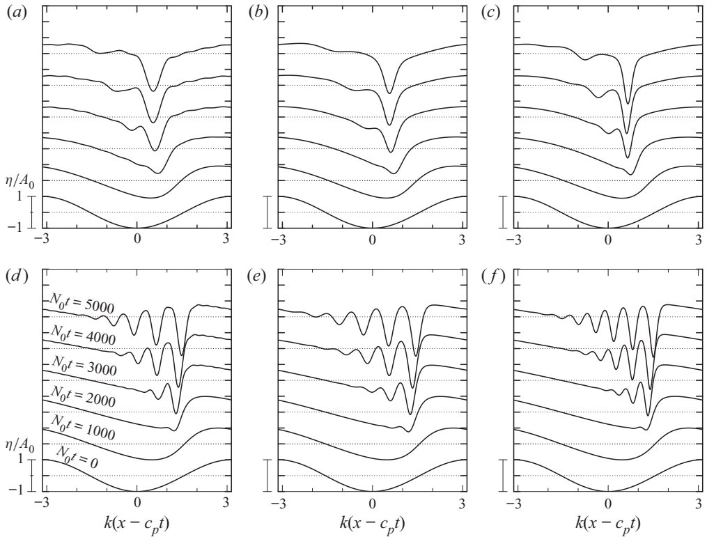
Figure 6. Comparison of vertical displacement predicted by (a,d) the superharmonic cascade (SHC) model, (b,e) the KdV-f equation, and (c,f) the MCC-f model, in cases with kH = 0.2 , A_0 = 0.003 and (a–c) f = 0.003N_0 , and (d–f) f = 0 . For SHC and KdV-f, the background stratification is exponential with N = N_0 at z_0 = -0.019H and d = 0.04H . For MCC-f, the equivalent parameters of the two-layer system are computed from the corresponding coefficients computed for the KdV-f equation. In all cases, the displacement is plotted at evenly spaced times, as indicated in (d), with successive times being vertically offset. The plots are given in a frame of reference moving with the phase speed c_p of the parent wave.
