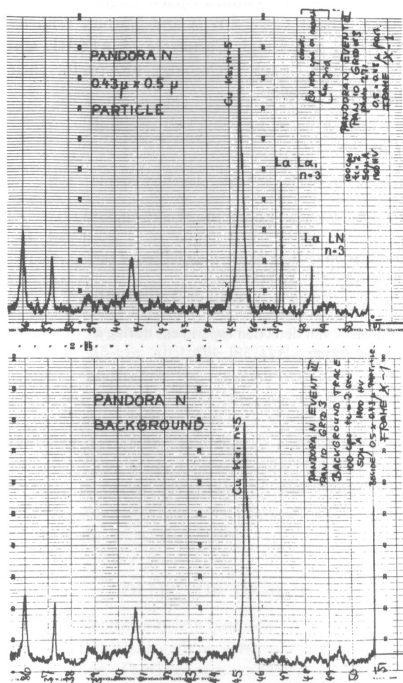
FIGURE 3.—X-ray spectra of a particle and nearby background.
