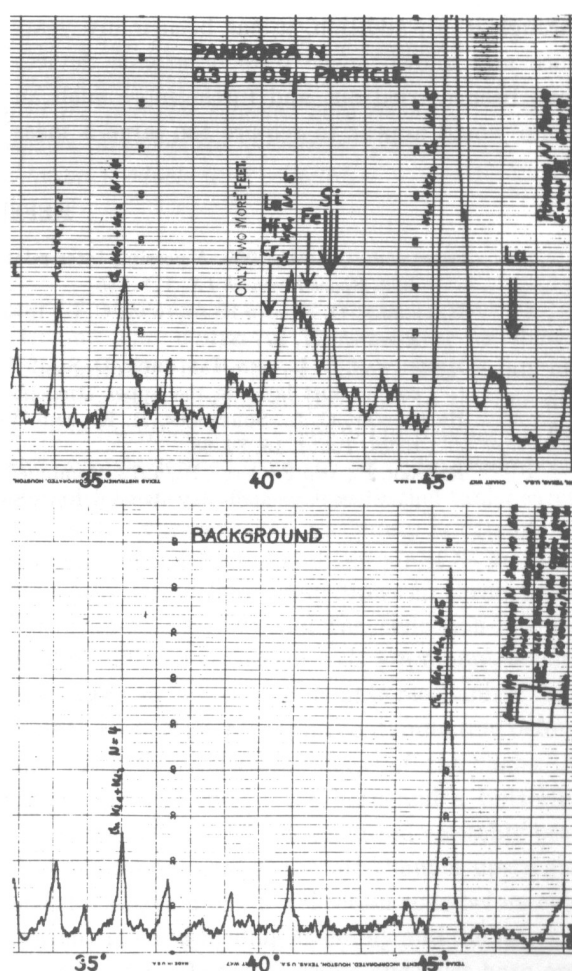
FIGURE 4.—X-ray spectra of a particle and nearby background.
