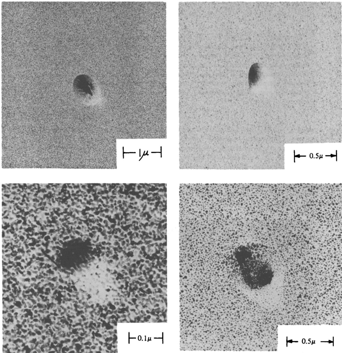
FIGURE 2.—Electron micrographs of noctilucent cloud particles collected.
