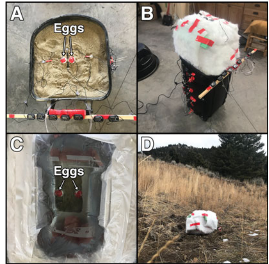
FIGURE 1. Photo series showing the surrogate dinosaur incubator, indoor sediment setup, and outdoor setup. The sediment container was 43 × 50 × 80 cm. The surrogate measured approximately 53 × 41 × 41 cm. A, A bird's-eye view of the sediment container, eggs, surface probes, and thermometer displays. In the final runs, the thermometer displays were localized and adhered to the side of the sediment container for ease of data capture. B, The surrogate—an insulated soft vinyl water container with water heater—on top of the sediment container. C, The eggs can be seen below the surrogate through the water held within the vinyl when the lid, insulation layer, and aquarium heater are removed (bird's-eye view). Tape covers the top to keep the thermometers in place within the eggs. D, An image of the surrogate outside in the testing area near Bozeman, Montana, at an elevation around 1850 m.
