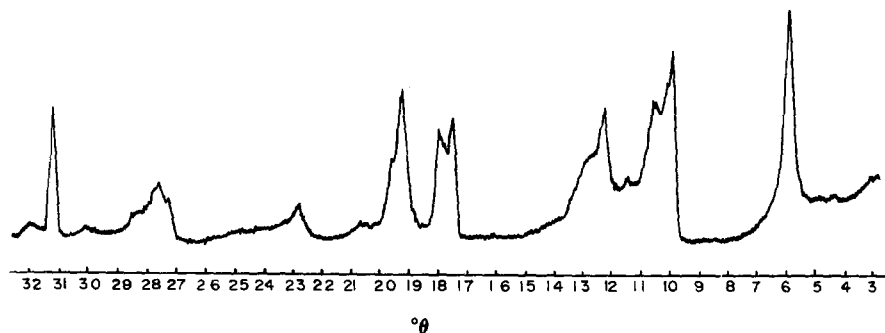
Fig. 1. X-ray diffractogram of a fully disoriented air-dried aggregate. d_{(001)} \approx 7.3 \text{ \AA} .
