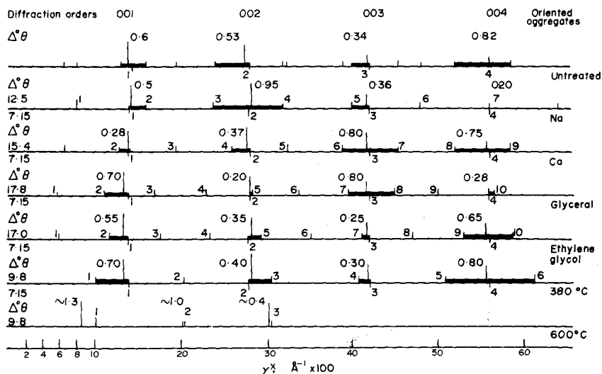
Fig. 3. Schematic representation of observed and theoretical (00l) orders in reciprocal space. Along each horizontal line are shown the positions of integral Bragg reflections from the separate components, e.g. 12.5 Å and 7.15 Å components. When these occur randomly intermixed, broad non-integral scattering maxima are likely to occur as indicated by the heavy lines. The positions and widths of the observed maxima are indicated.
