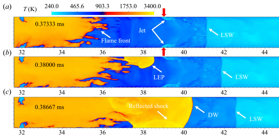
Figure 42. Snapshot of temperature contour before and after DDT in the z -direction. LSW – leading shock wave, LEP – localized explosion point, DW – detonation wave.
