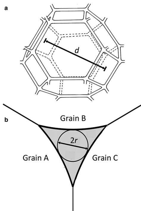
Fig. 1. (a) Network of melt veins (like that considered by Frank (1968)) approximated by truncated semiregular octahedra (modified from Dani and others, 2012). (b) Cross-section of a water vein at a three-grain intersection, with vein radius, r , describing the size of an equilateral triangle used to model Poiseuille flow through veins.
