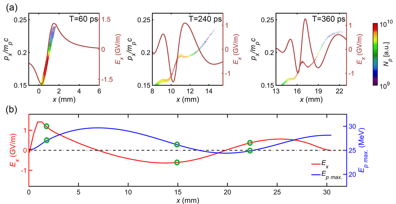
Figure 4. (a) Snapshots of proton distributions in phase space ( x, p_x ) and the longitudinal electric field at 60, 240 and 360 ps, in a single-stage HC. (b) Longitudinal electric field (red curve) in the coordinate frame of the traveling highest-energy protons, and the evolution of the cut-off energy (blue curve) in a single-stage HC, where the three groups of green circles mark the three statuses in (a).
