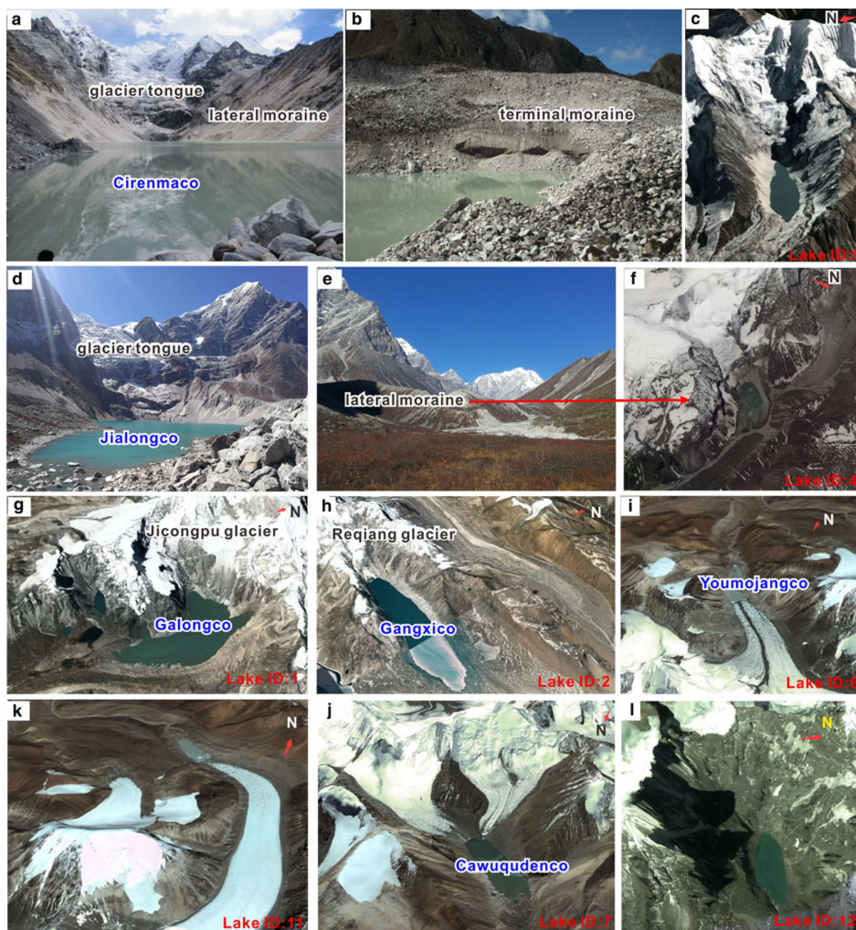
Fig. 6. Ground and 3-D views of eight PDGLs. (a, b) Photos for Cirenmaco (taken by W. Wang on 21 September 2012); (c) Cirenmaco from Google Earth image on 25 November 2016. (d, e) Photos for Jialongco (taken by G. Zhang on 18 October 2017); (f–i) Jialongco, Galongco, Gangxico, Youmojangco, Lake no. 11 from Google Earth images on 5 June 2015, 10 October 2017, 10 October 2017, 01 November 2012 and 01 November 2012, respectively. (k–l) Cawuqudenco and Lake no. 12 from Google Earth images on 01 November 2012 and 28 November 2009, respectively. Source of Google Earth images is from DigitalGlobe. The numbers displayed in red refer to the ID of the lakes listed in Table 4.
