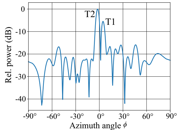
Figure 10. Cross-sectional view derived from Fig. 9 at R = 3.7 m. The two targets are visible as two distinct peaks with a 3-dB width of 3.5^\circ . Due to alignment inaccuracy, the peaks are shifted 1.2^\circ off center.
