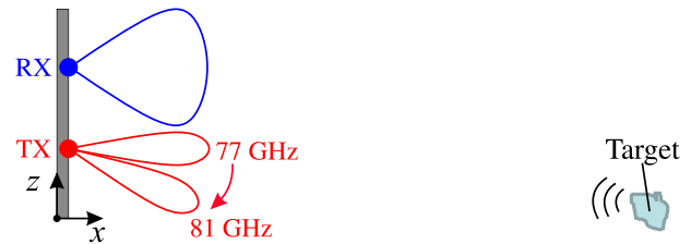
Figure 2. Sketch of the TX and RX antenna patterns when considering the system in a side view. The RX antennas have a wide beam that remains rather constant throughout the frequency chirp. The main lobe of the TX antennas is continuously tilted downward during the chirp. A target is detected during a certain part of the frequency ramp. The information about the target angle is contained in the amplitude of the intermediate frequency signal.
