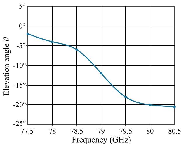
Figure 7. Main lobe direction of the combined pattern dependent on frequency, derived from Fig. 6. This figure serves as a frequency-dependent angular reference for determining \theta .
