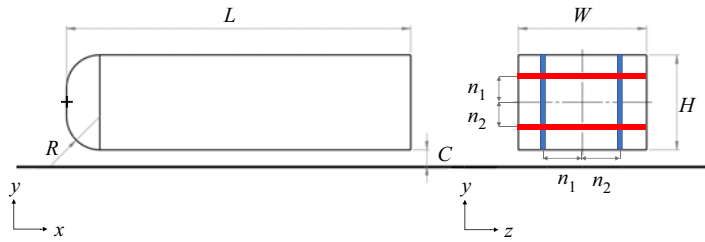
Figure 1. Square-back Ahmed body scaled by one fourth, with width W = 97.25 mm (drawing scale 1:2). Pressure sensors on the base are marked by the blue and red lines in the vertical ( y ) and the horizontal ( z ) directions, respectively. Point (0, 0, 0) is positioned at the centre of the front surface indicated with the black + .
