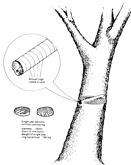
FIG 3 A CORE EXTRACTED FROM A BORING ACROSS A FULL DIAMETER AND ITS BREAK-UP INTO ANNUAL SECTIONS
