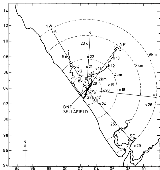
FIG 4. HAWTHORN BERRY SAMPLING SITES, OCTOBER 1981
