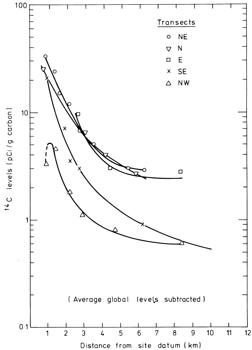
FIG 5. PRELIMINARY DISPERSION PATTERN DATA FOR 5 TRANSECTS OF THE 1981 HAWTHORN BERRY SURVEY
