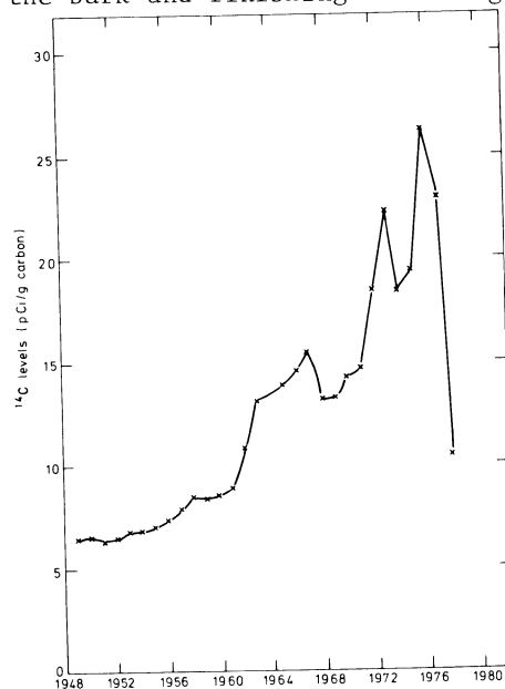
FIG 2 ^{14}\text{C} LEVELS FROM TREE RINGS OF A SYCAMORE TREE NEAR SELLAFIELD
