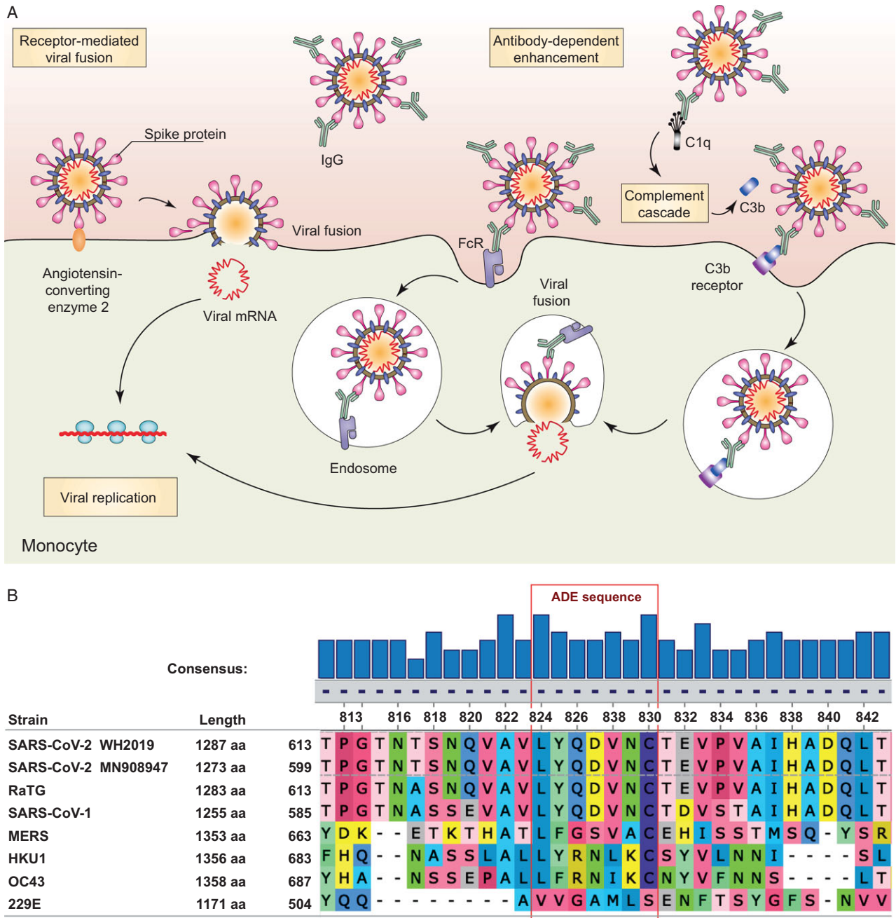
Fig. 1. Antibody-dependent enhancement (ADE). (A) Mechanism – normal viral fusion occurs with binding of the coronavirus spike protein to its receptor, the angiotensin-converting enzyme 2 protein (ACE2). This induces a conformational change in the S protein, exposing a membrane fusion domain, resulting in viral fusion and mRNA release into the cell. With ADE, antibody binding to the S-protein both facilitates cell binding via the FcR and induces a conformational change in the spike protein exposing the fusion domain. A similar process can occur if the IgG binds complement, with the C3b:IgG:virus complex being taken up via the C3b receptor. (B) The ADE-associated spike glycoprotein peptide sequences S579-603 from SARS [12] are also conserved in SARS-CoV-2 strains (bold) and the closely related bat CoV strain (RaTG). There is less sequence homology in MERS and the common human CoV strains (HKU1, OC43, 229 E). Sequence homologies analyzed with the Clustal Omega method using Unipro UGENE v33.0 software.
