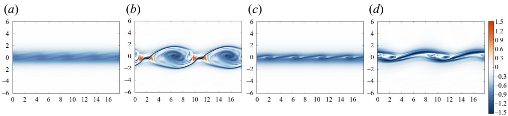
Figure 16. Vorticity at Re = 1000 and Pr = 7 at t = 100 . For (a) Ri_b = 0.1 , k = k_2 , (b) Ri_b = 0.1 , k = k_1 , (c) Ri_b = 0.3 , k = k_2 , (d) Ri_b = 0.3 , k = k_1 .
