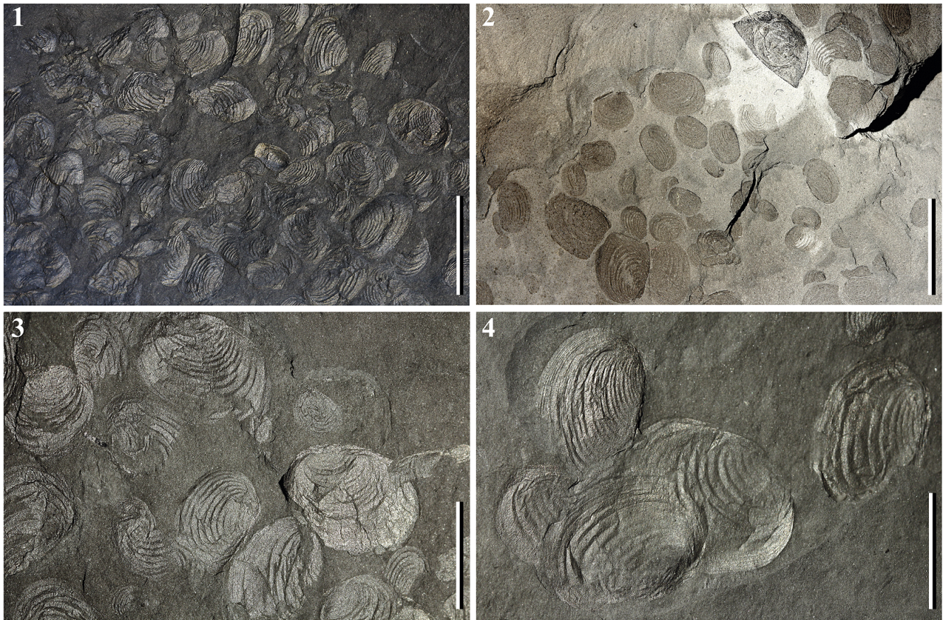
Figure 2. Examples from the Consthurn clam shrimp mass layer. (1) Detail from slab EIB552b; note associated lingulid brachiopod near center. (2) Detail from slab EIB549a; note associated head shield of the eurypterid Adelophthalmus sievertsi (Størmer, 1969) (upper right), crossed polarizing filters. (3) Detail from slab EIB552a; note differences in size and form of dorsal margin. (4) Detail from slab EIB551a; note differences in the spacing of growth lines. (1, 2) Scale bars = 10 mm; (3, 4) scale bars = 5 mm.
